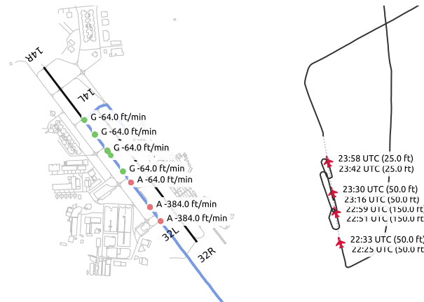
Figure 2. (Left) Flight DLH83K on 25 February 2017: it is very difficult to determine the exact landing point: the onground flag was activated after the vertical rate came close to zero. A long landing in this situation is not unreasonable, but these data cannot reasonably support this hypothesis. (Right) No onground flag is activated, but the trajectory of aircraft identifier ae0455 on 14 September 2020 suggests landing practice activity on an aircraft carrier off California.
