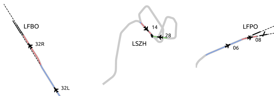
Figure 4. Successive runway alignments may suggest different situations depending on the configuration of the airport and on the vertical speed: runway change with parallel runways at Toulouse LFB0 airport on the left, failed landing attempts with go-around at Zürich LSZH airport in the middle or circle to land manoeuvres at Paris–Orly LFP0 airport.
