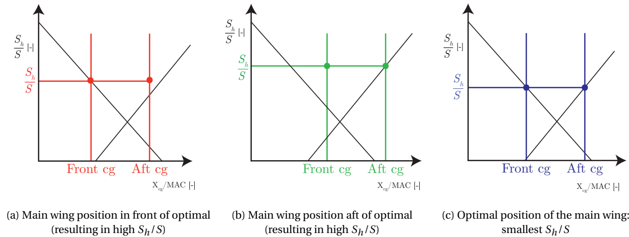
Figure 5.34: Varying main wing longitudinal position, changing cg-range and determining S_h/S
