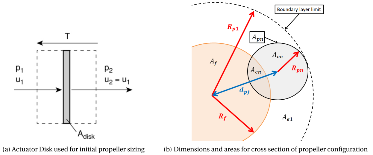
Figure 5.11: Propulsion theory setup
