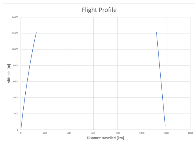
Figure 7.1: The flight profile of the Greenliner
