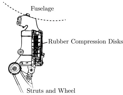
Figure 5.39: Shock absorber placement, adapted from [18]
