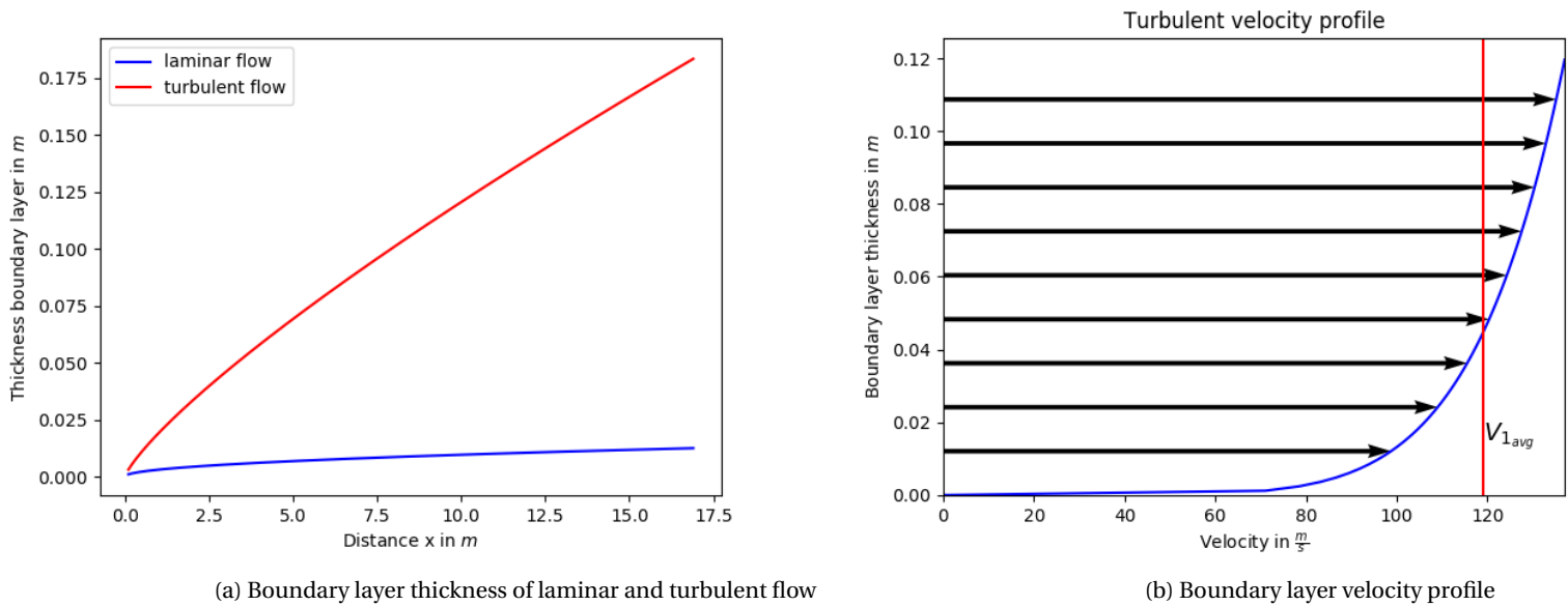
Figure 5.8: Boundary layer thickness and velocity overview
