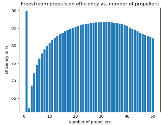
(b) Efficiency vs. number of propellers
