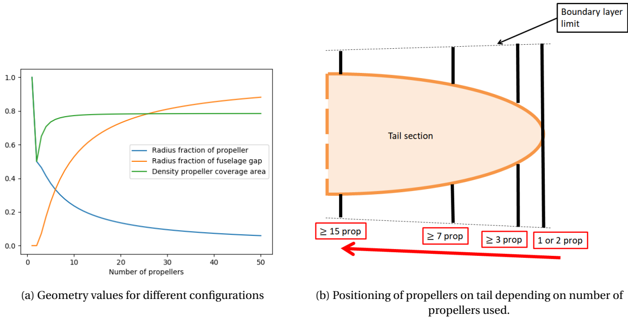
Figure 5.10: Geometry setup
