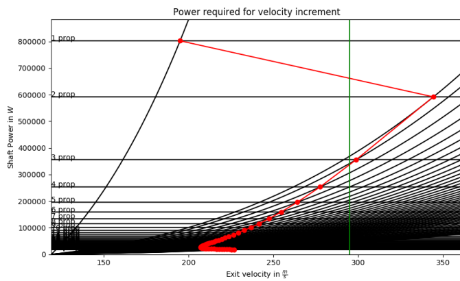
(a) Power curves to calculate exhaust velocity
