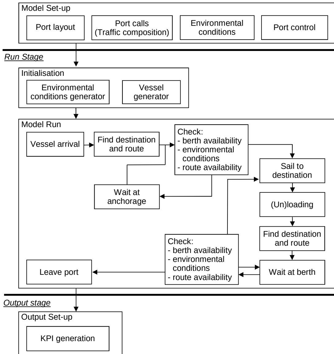
Figure 6.2: Model structure (adapted from Macquart, 2017).
