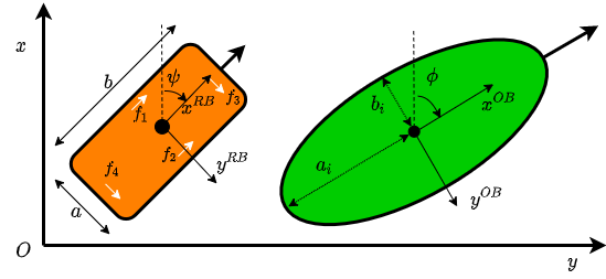
Fig. 4: The Roboat and an obstacle vessel. Angles \psi and \phi denote the orientation of the boats. a and b are the width and the length of the Roboat. a_i and b_i are the semi-major and minor axis respectively of obstacle boat i . The Roboat’s thrusters can exert force f in two directions, the white arrows denote the positive direction.
