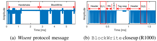
Fig. 1. State of the art (C)RFID downstream protocol ( Wisent [5]) trace by custom-made EPC C1G2 [6] sniffer. Setup: Impinj R1000 reader (3.2.4.240 firmware), WISP 5.1. We notice large overheads due to: (a) Wisent protocol itself (handshake every EPC C1G2 data frame: BlockWrite )—48% overhead, and (b) limitations of Impinj R1000 firmware (unnecessary slicing of BlockWrite into parts, marked as D(x) ; RN: tag handle)—85% overhead. Delay between \approx(1,3) ms in (a), is also due to Impinj firmware.
