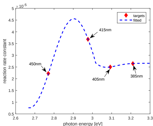
Figure 3.6: Fitted model of the reaction rate constants as a function of the photon energy. The arrows indicate the experimenting light sources. The simulated range of the photon energy 2.7 \sim 3.3\text{eV} corresponds to the wavelength range of 375 \sim 460\text{nm} .
