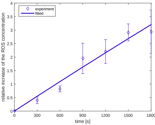
Figure 3.5: Fitted curve to the measured relative ROS concentration data from the 415nm light irradiation experiment.
