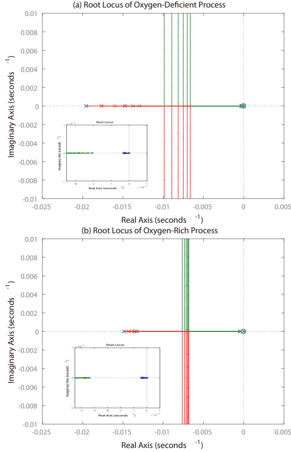
Figure 6.2: The root locus plots of the seven linearized MSO processes at different equilibrium points: (a) ^3\text{O}_2 deficient case, (b) ^3\text{O}_2 rich case. The scales of the corresponding axes in the two figures are the same. The inserts in the figures show the cancellation of the pole s = 0 with the zero.
