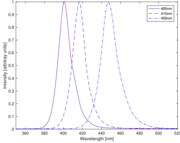
Figure 2.1: The measuring results of the actual wavelengths of 405-nm, 415-nm and 450-nm.
