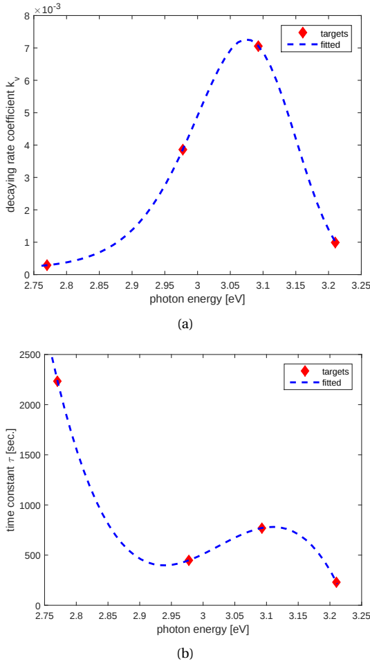
Figure 3.9: Fitted model of k_v and \tau as a function of the photon energy: (a) k_v as in Eq. (3.7), (b) \tau as in Eq. (3.8).
