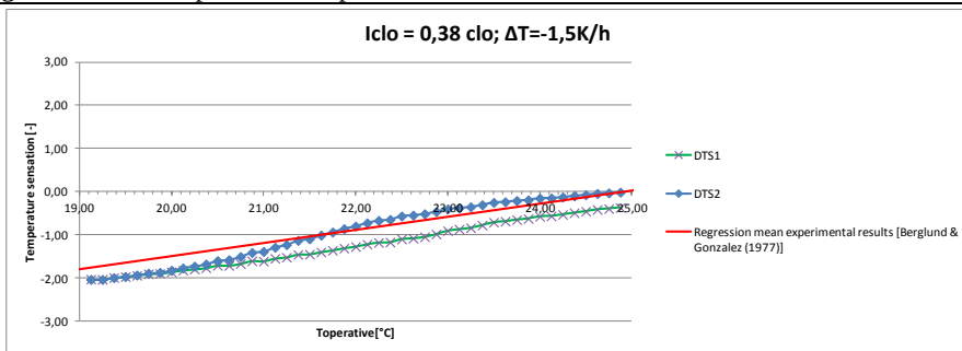
Figure 2.3.14. Temperature ramp \Delta T = -1.5 K/h , I_{clo_{intrinsic}} = 0.38 .
