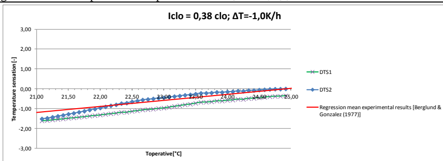
Figure 2.3.13. Temperature ramp \Delta T = -1.0 K/h , I_{clo_{intrinsic}} = 0.38 .
