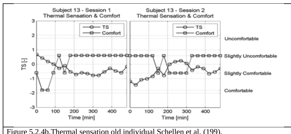
Figure 5.2.4b. Thermal sensation old individual Schellen et al. (199).
