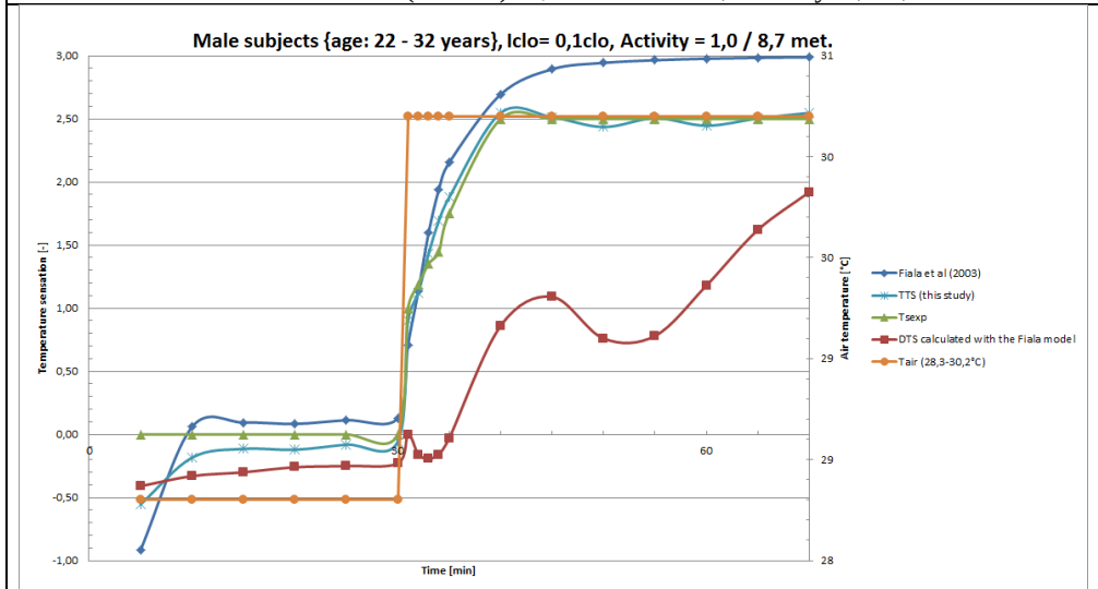
Figure 2.4.8. Calculation results ( TTS_{\text{physical}} ) versus experimental results and the DTS-model of Fiala et al. (19) in combination with the Stolwijk model (dark blue line) and the DTS calculated with the Fiala human model (red line). T_{\text{air}} : 28.3-30.2°C; Activity: 1,0-8,7 met.
