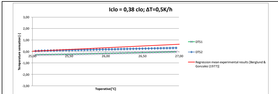
Figure 2.3.9. Temperature ramp \Delta T=0.5 K/h, \text{Iclo}_{\text{intrinsic}} = 0.38 .
