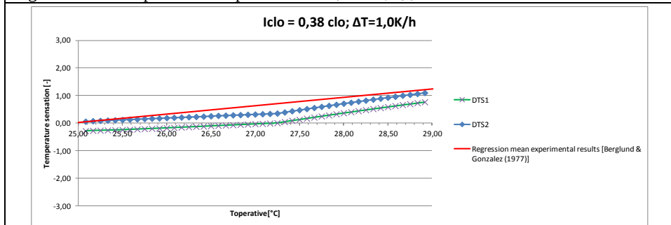
Figure 2.3.10. Temperature ramp \Delta T=1.0 K/h, \text{Iclo}_{\text{intrinsic}} = 0.38 .
