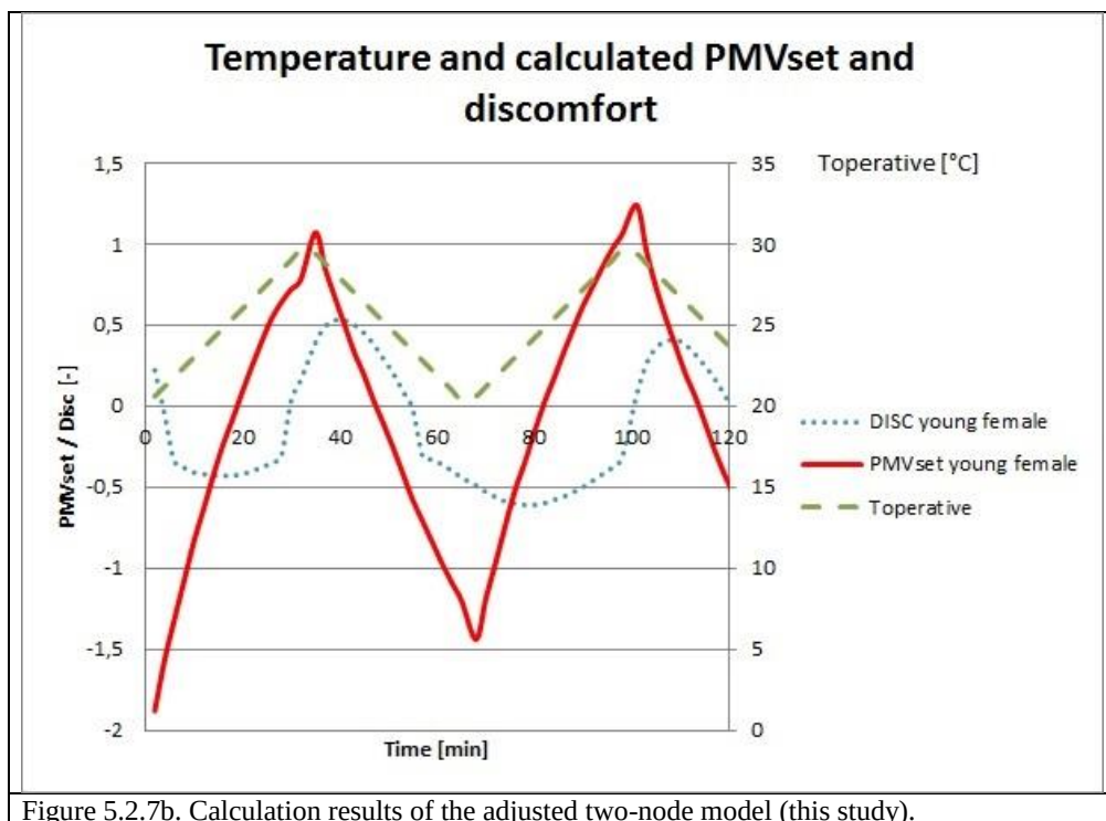
Figure 5.2.7b. Calculation results of the adjusted two-node model (this study).
