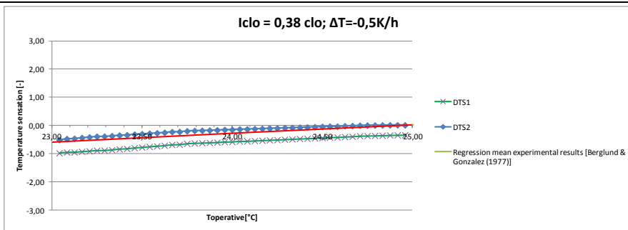
Figure 2.3.12. Temperature ramp \Delta T = -0.5 K/h , I_{clo_{intrinsic}} = 0.38 .
