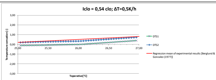
Figure 2.3.15. Temperature ramp \Delta T = 0.5 K/h , I_{clo_{intrinsic}} = 0.54 .
