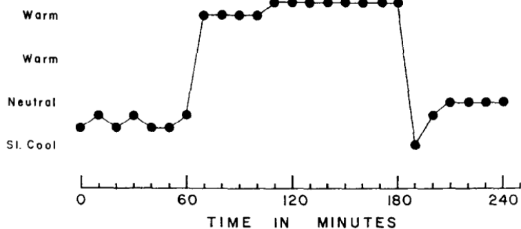
Figure 2.3.5. V_{air}=0.05 m/s, I_{clo}=0 . Neutral: 28.1^{\circ}\text{C}/\text{RH}=43\% , Warm: 47.8^{\circ}\text{C}/\text{RH}=27\% , Neutral: 28.3^{\circ}\text{C}/\text{RH}=44\% (115).
