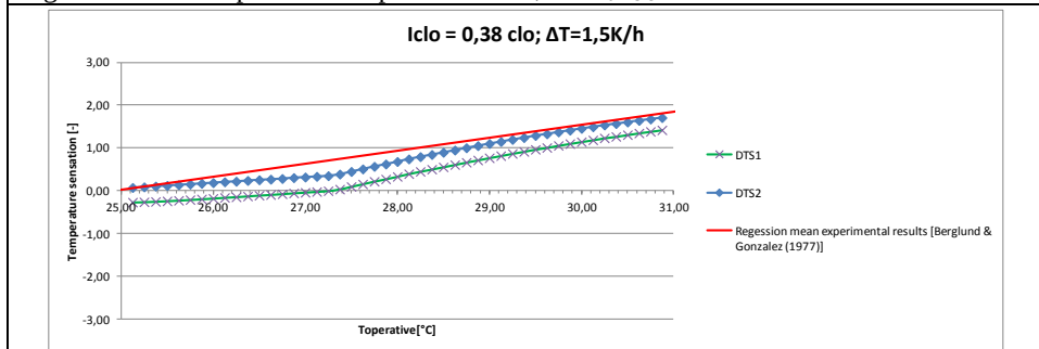
Figure 2.3.11. Temperature ramp \Delta T=1.5 K/h, \text{Iclo}_{\text{intrinsic}} = 0.38 .
