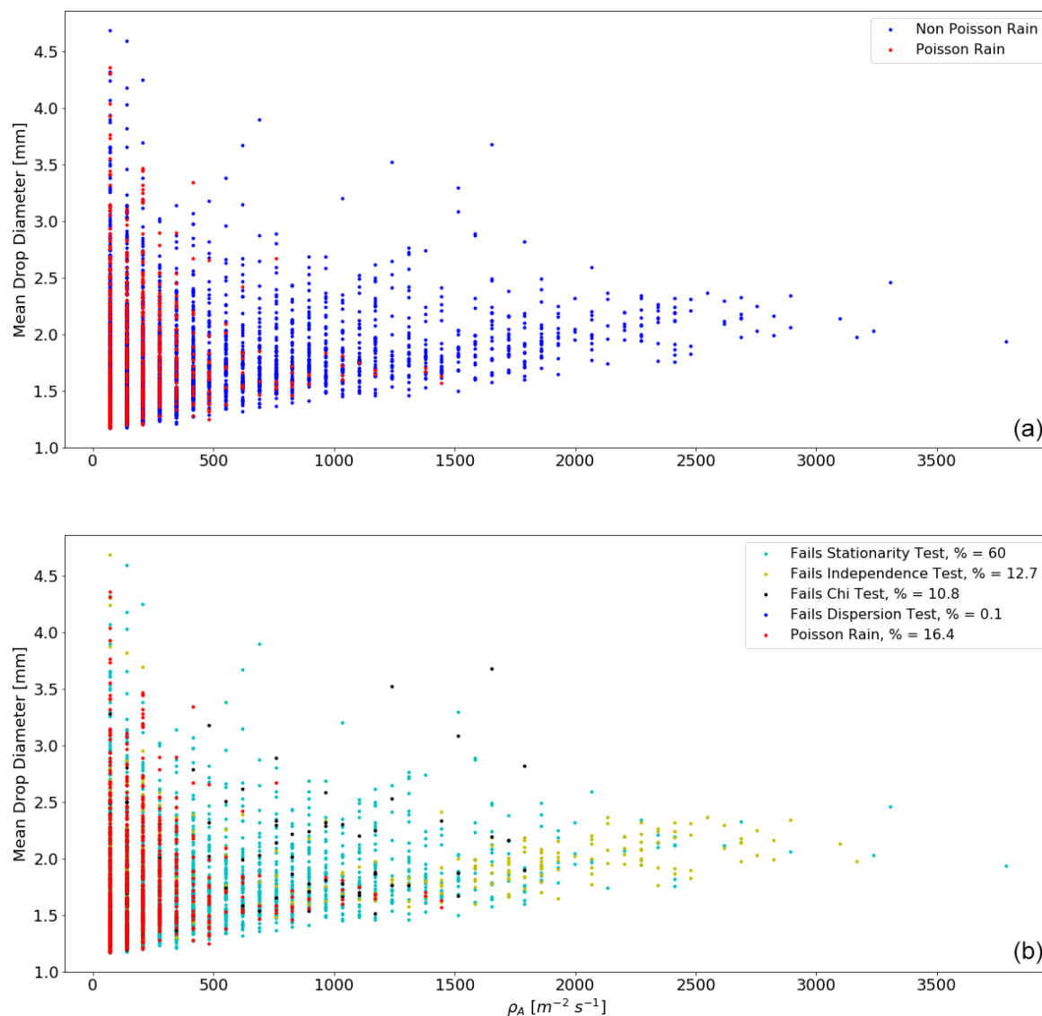
Figure 9. Trends in mean drop size for Poisson and non-Poisson rain are presented as well as the percentage of drops that fail each of the Poisson tests. Panel (a) differentiates between Poisson and non-Poisson rain. Panel (b) is further subdivided to show which of the Poisson tests each data point fails.
