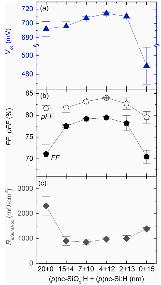
Fig. 9. Front junction FBC-SHJ solar cells with varying thicknesses of (p)-contact ((p)nc-SiO x :H + (p)nc-Si:H): (a) V_{oc} ; (b) FF and pFF ; (c) R_{s,SunsVoc} . Solar cells feature a nominal 4.4% front metal coverage. The results represent averaged parameters from three solar cells. The error bars represent the standard deviations.
