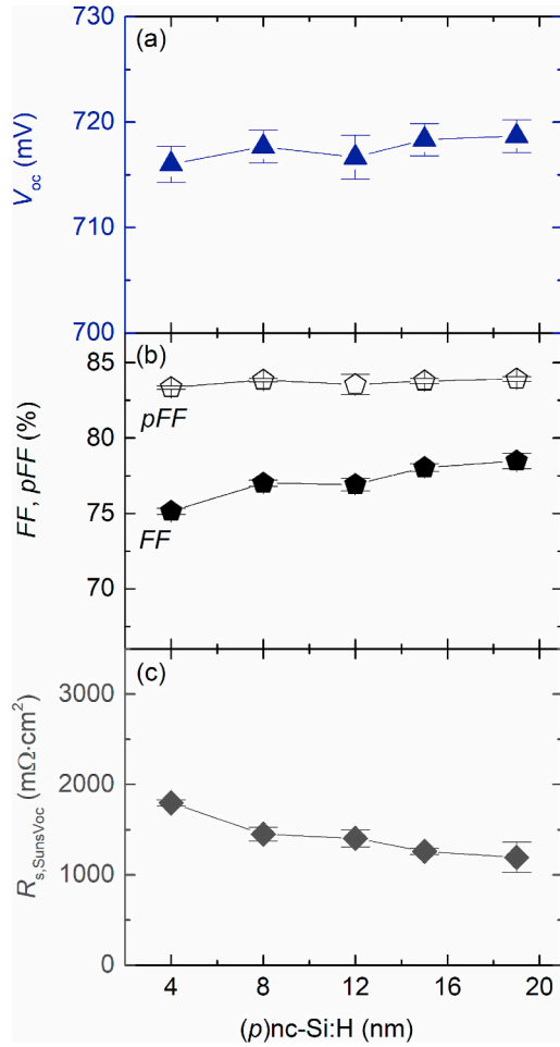
Fig. 10. Rear junction FBC-SHJ solar cells with (p)-contacts featuring a fixed 4-nm thick (p)nc-SiO x :H but varying (p)nc-Si:H layer thicknesses: (a) V_{oc} ; (b) FF and pFF ; (c) R_{s,SunsVoc} . Solar cells feature a nominal 4.4% metal coverage. The results represent averaged parameters from three solar cells. The error bars represent the standard deviations.
