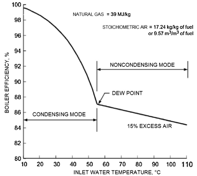
Fig. 2. Effect of return (inlet) temperature on efficiency of condensing boilers [39].
