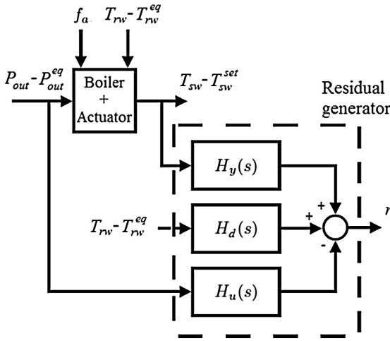
Fig. 4. Residual generator.
