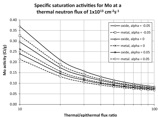
Fig. 1 Specific saturation activities to be expected in an irradiation facility with a thermal neutron flux of 1 \times 10^{13} \text{ cm}^{-2} \text{ s}^{-1} , as a function of the thermal/epithermal flux ratio, for various values of \alpha and for the two sample types, as calculated with Eqs. 14 and 15 in this paper
