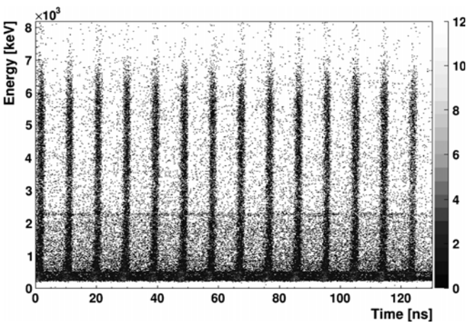
Figure 4: Timing spectrum for 225 MeV protons hitting a water phantom with a pulse period of 9.4 ns, as measured with the LaBr 3 :Ce scintillator of the Compton camera.
