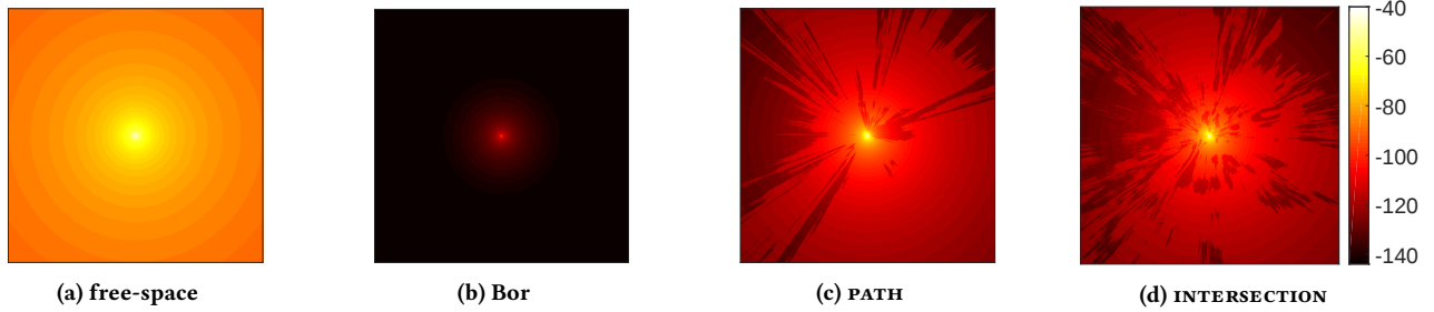
Figure 19: ESP prediction on a 6 \times 6 km 2 area centered in G_8 .
