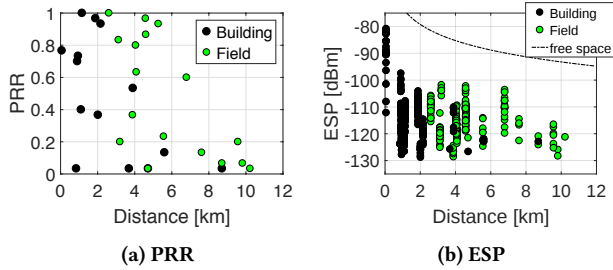
Figure 12: Reliability and power vs. distance for BUILDING and FIELD dominated links.
