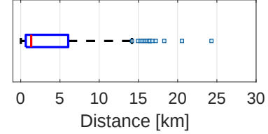
Figure 4: Variation of communication ranges for LoRa links.
