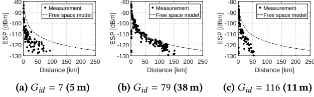
Figure 3: ESP vs. distance for selected gateways.
