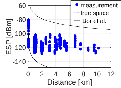
Figure 14: ESP vs. distance for measurements (dots), free-space model (dashed line) and Bor's model (solid line).
