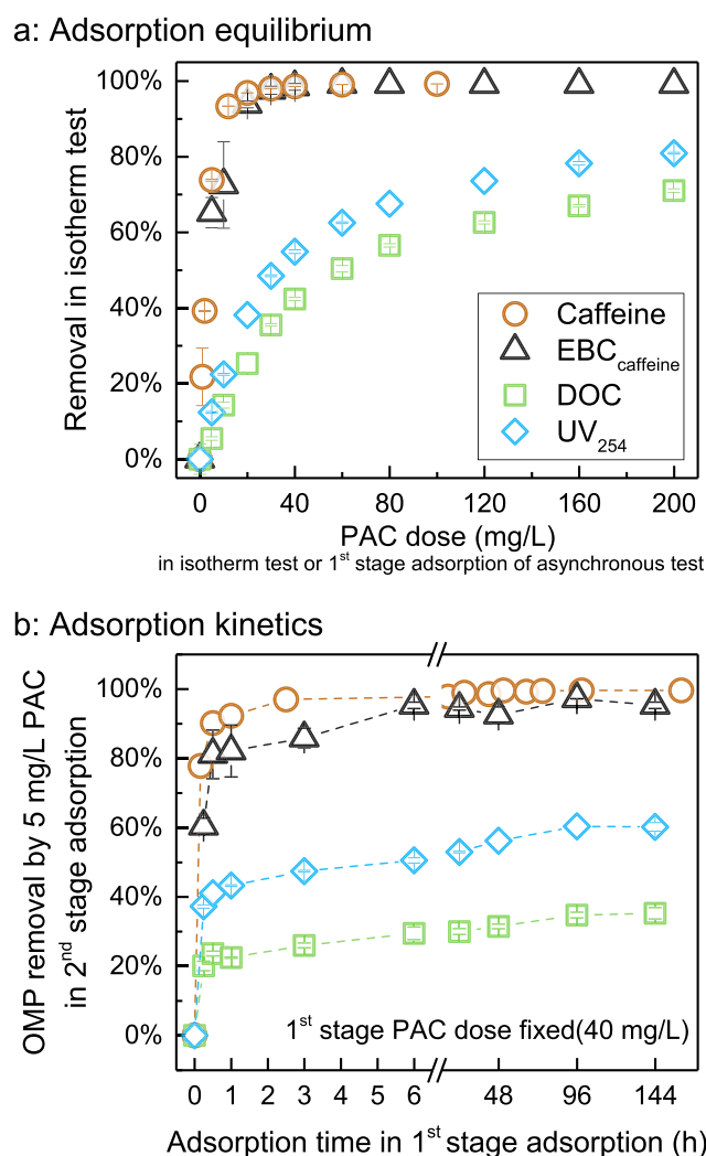
Fig. 6. The removal of DOM competitor (fictive-EBC, sum parameters including DOC and UV 254 ) in the first stage of DOM-OMP asynchronous adsorption as compared to removal of caffeine in isotherm/kinetic test in untreated water at (a) adsorption equilibrium; (b) adsorption kinetics with 40 mg PAC/L. Note that second stage adsorption were all in 7 d; EBC removal calculation was based on fixed K_{F,EBC} (21.84 (nmol/mg)/(nmol/L) 1/n ) and 1/ n_{EBC} (0.69).
