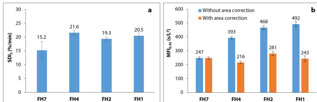
Fig. 11. SDI 3 (a) and MFI 0.45 (b) values measured with various filter holders (n = 10). DCW1. CA filter.
