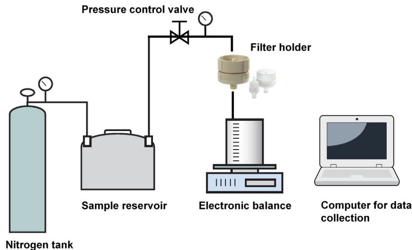
Fig. 3. Constant pressure, dead-end, filtration setup.
