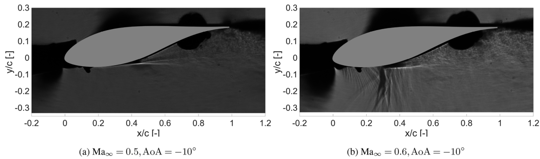
Figure 9. Instantaneous schlieren images showing no shock waves in panel (a), while clear shock waves appear in panel (b) between x/c = 0.2 – 0.4 .
