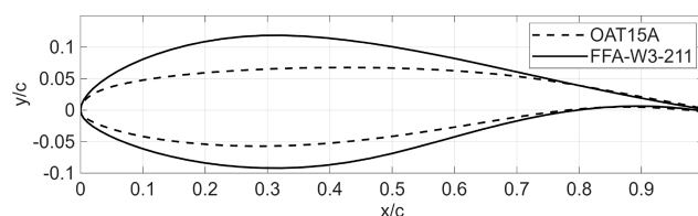
Figure 1. Comparison of the OAT 15A supercritical airfoil (dashed line) and the FFA-W3-211 wind turbine airfoil (solid line).
