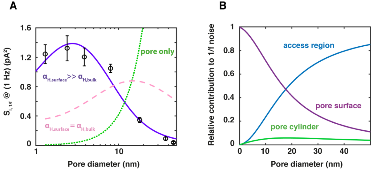
Figure 3. (A) Low-frequency 1/f noise plotted as a function of the pore diameter (black circles). We observe a decreasing trend of 1/f noise with increasing nanopore size, which spans more than one order of magnitude over the analyzed pore diameter range. Error bars represent standard deviations. The three lines represent model fits to the nanopore data: The green dotted line accounts for the model with no access resistance contribution; pink dashed line includes the access resistance, but treats 1/f noise as coming from one mechanism with a single Hooge parameter; and the purple curve shows the model comprising the access resistance and two independent Hooge parameters associated with bulk and surface noise. (B) Relative
