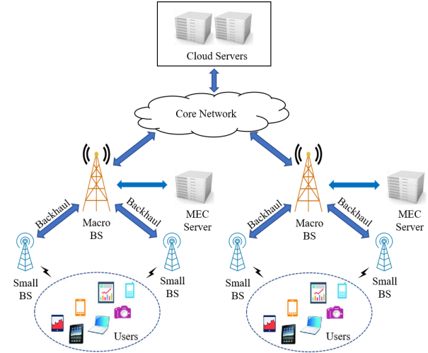
Fig. 1: MEC Architecture with localized service area.
