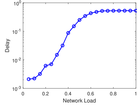
Fig. 3: GPON Delay
