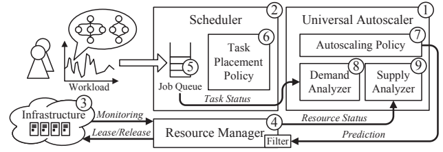
Figure 1: Elastic cloud platform.
