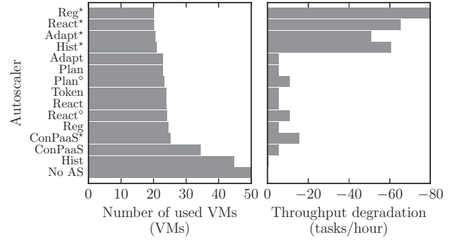
Figure 8: The average number of used VMs during the experiment and the average throughput degradation (compared with the no autoscaler case). All results are given for Workload 1.
