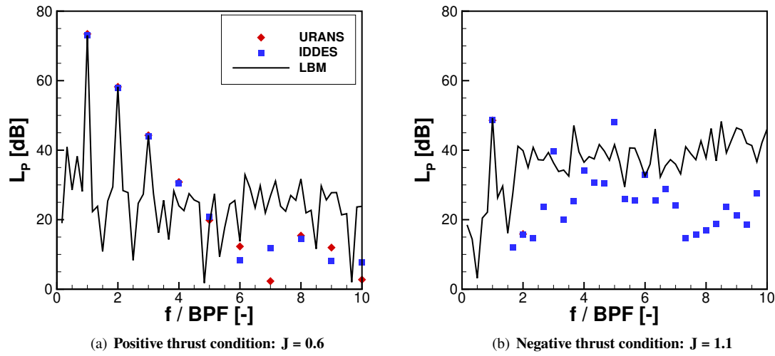
Fig. 10 FFT analysis at \Theta = 90^\circ .
