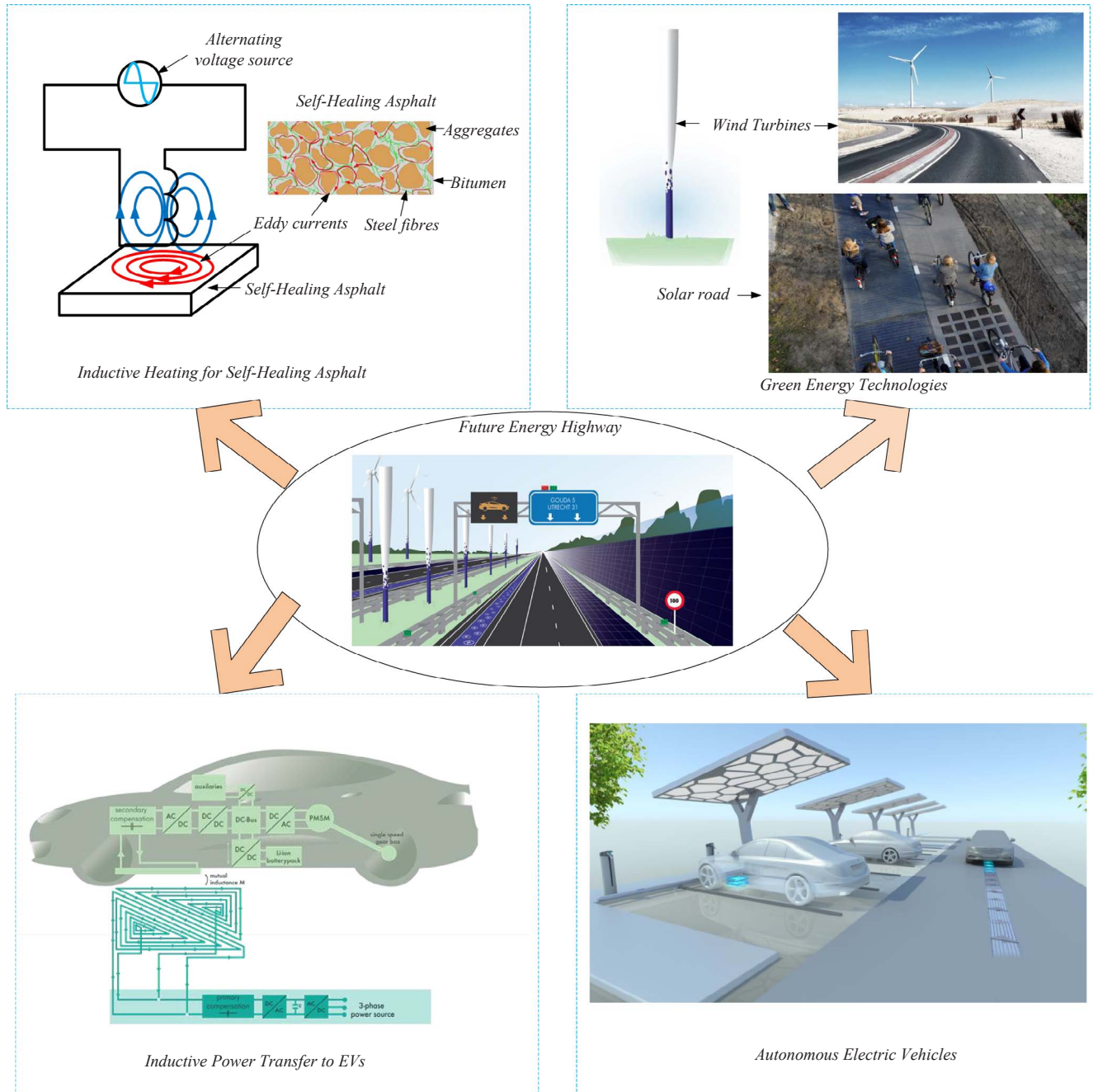
Fig. 1. Future energy highway integrating inductive coils for both inductive power transfer and induction heating, with green energy technologies for (autonomous) electric mobility.
