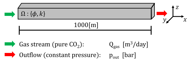
Fig. 1 One dimensional domain setup. Constant injection rate on the left boundary (Neumann) and constant pressure (Dirichlet) on the right. The lateral (y-direction) and vertical (z-direction) dimensions of the domain are 1[m]
