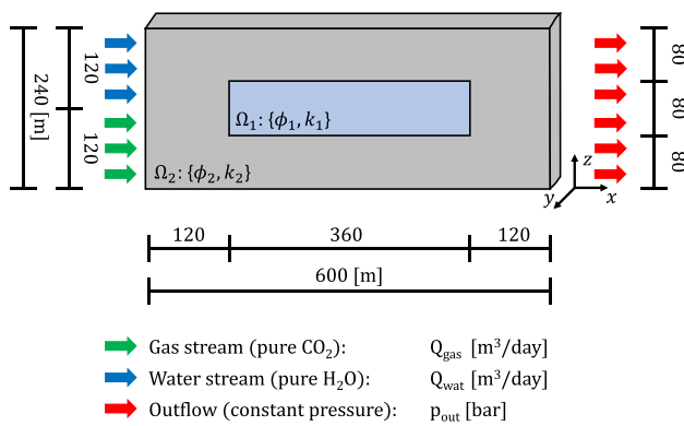
Fig. 2 Configuration of the 2D test case (Section 4.2). Constant injection rate on the left boundary (Neumann) and constant pressure (Dirichlet) on the right. The lateral y -direction of the domain is 10m
