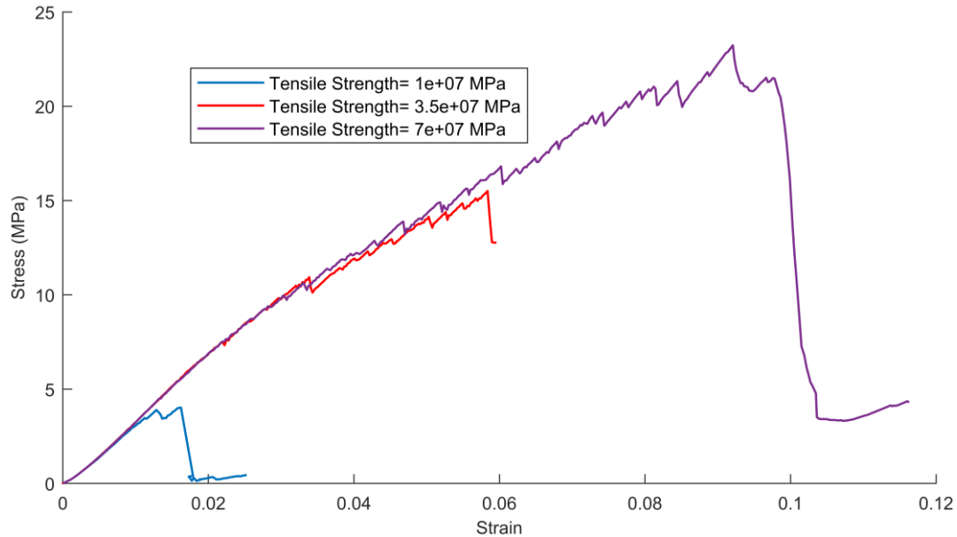
Figure 7: Effect of tensile strength on the stress-strain curve of EBPM
