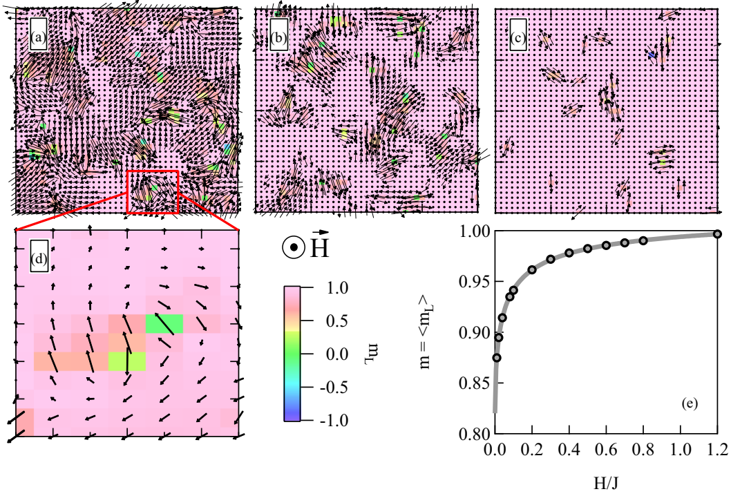
FIG. 5. Outcome of the Monte Carlo simulations for an antiferromagnetic bond concentration of 5%. [(a)–(c)] Simulated spin maps for H/J = 0.01 , 0.1 , and 0.8 , respectively, where J is the first-neighbor exchange term. We display portions of 40 \times 40 spins for clarity. The longitudinal magnetization m_L (i.e., parallel to the applied field) is color-coded while the arrows represent the transverse component m_T . (d) Example of a vortexlike chiral spin circulation stabilized at H = 0.01 J. (e) Field dependence of the bulk magnetization m , defined as the average value of the longitudinal magnetization per spin \langle m_L \rangle .
