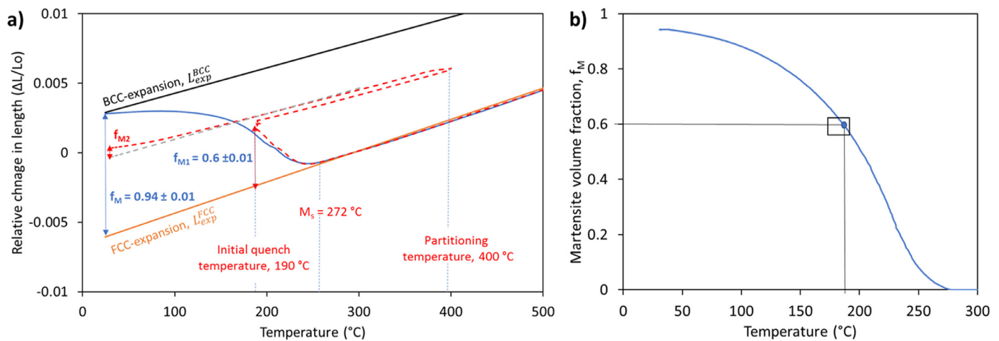
Fig. 2. (a) Relative change in length versus temperature of an as-quenched (solid blue line) and QP400-3600 (dashed red line) specimens. f_M is the volume fraction of martensite formed after an as-quench heat treatment; f_{M1} and f_{M2} are the volume fractions of primary and fresh martensite formed during QP400-3600 heat treatment, respectively (b) Volume fraction of martensite as a function of temperature obtained applying the lever rule to the as-quench dilatation curve.
