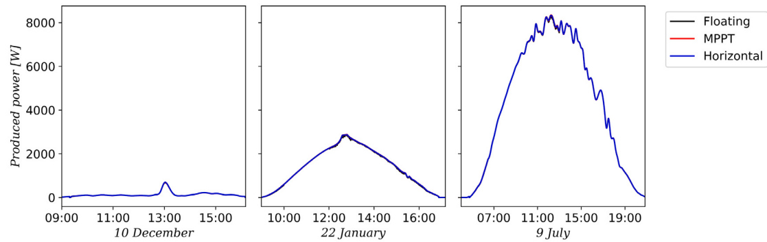
Fig. 13. Plot of the power produced by the floating, MPPT, and horizontal PLS-NF25 systems on selected days. December 10th is a cloudy windy winter day; January 22nd is a sunny not windy winter day; and July 9th is a sunny windy summer day.
