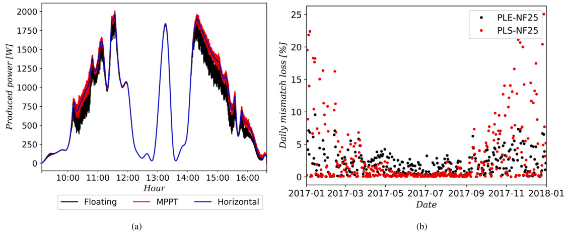
Fig. 15. (a) Plot of the power produced by the floating, MPPT, and horizontal PLE-NF25 systems on January 14th, the day with the highest daily mismatch losses. (b) Daily mismatch throughout the year for PLE-NF25 and PLS-NF25.
