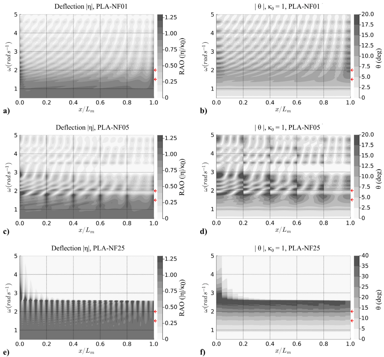
Fig. 7. Contour plots of the structural response along the length of the platform for ocean-wave frequency in range \omega \in [0.7, 5.0] . (a-b) Magnitude of deflection and slope for PLA-NF01. (c-d) Magnitude of deflection and slope for PLA-NF05. (e-f) Magnitude of deflection and slope for PLA-NF25. The arrows indicate the two frequencies that were plotted in Fig. 6.
