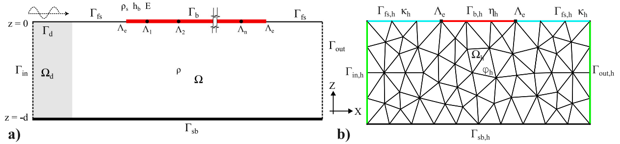
Fig. 1. (a) Schematic of the boundary value problem, consisting of the fluid domain \Omega with constant water-depth d , bounded by the bottom \Gamma_{sb} , inlet \Gamma_{in} , outlet \Gamma_{out} , free-surface \Gamma_{fs} and the floating PV platform \Gamma_b . Here \Lambda_j represent the free-hinges in the floating PV platform. (b) Sketch of the discretized geometric entities, with \Omega_h representing the discretized fluid domain, and \Gamma_{sb,h} , \Gamma_{in,h} , \Gamma_{out,h} , \Gamma_{fs,h} and \Gamma_{b,h} representing the discretized boundaries. Consequently, \phi_h , \eta_h and \kappa_h are the discrete solutions to the velocity potential, free-surface elevation and beam deflection, respectively.
