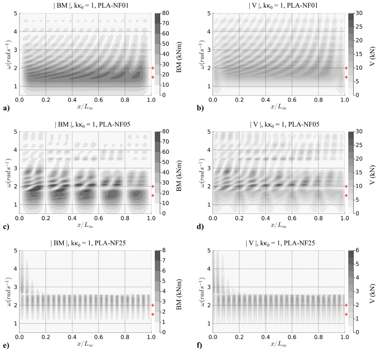
Fig. 8. Contour plots of the structural response along the length of the platform for ocean-wave frequency in range \omega \in [0.7, 5.0] . (a–b) Magnitude of bending moment and shear force for PLA-NF01. (c–d) Magnitude of bending moment and shear force slope for PLA-NF05. (e–f) Magnitude of bending moment and shear force for PLA-NF25. The arrows indicate the two frequencies that were plotted in Fig. 6.
