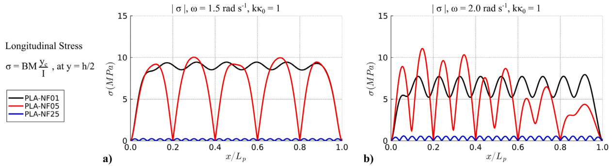
Fig. 6. Plots of the structural response of PLA-NF01, PLA-NF05 and PLA-NF25 floating platforms to monochromatic ocean-wave excitation of \omega = 1.5 \text{ rad s}^{-1} and \omega = 2.0 \text{ rad s}^{-1} . (a-b) Magnitude of longitudinal stress in the cross-section, at y_c = h_b/2 . Here y_c is the normal distance between the rotation axis for bending and the location on the cross-section.
