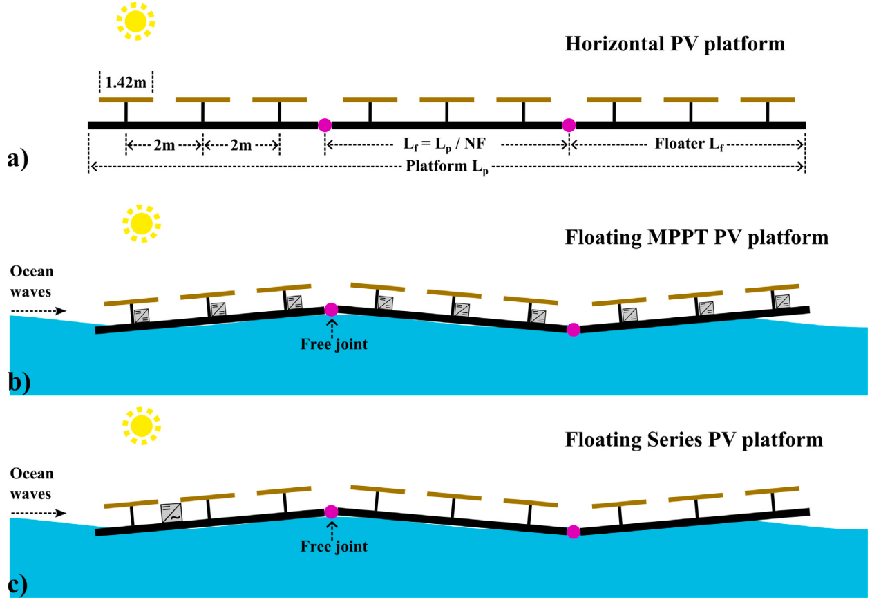
Fig. 3. Schematic of the floating PV platform. (a) Horizontal PV platform not subjected to the movement of waves. (b) Floating PV platform, with individual optimizers containing an MPP tracker and a DC-DC converter for each PV module. (c) Floating PV platform with all the modules connected in series and a single central inverter.
