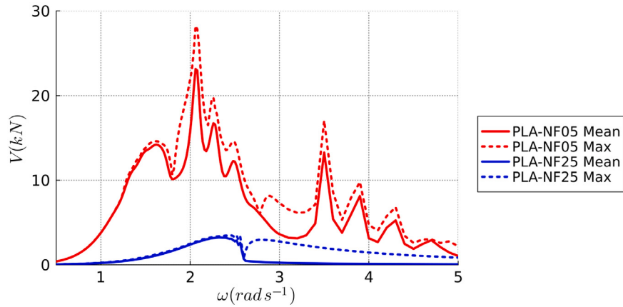
Fig. 10. Plot of the maximum and average values of the magnitude of shear force |V| at the joints of cases PLA-NF05 and PLA-NF25, for unit beam-width and unit-slope wave excitation.
