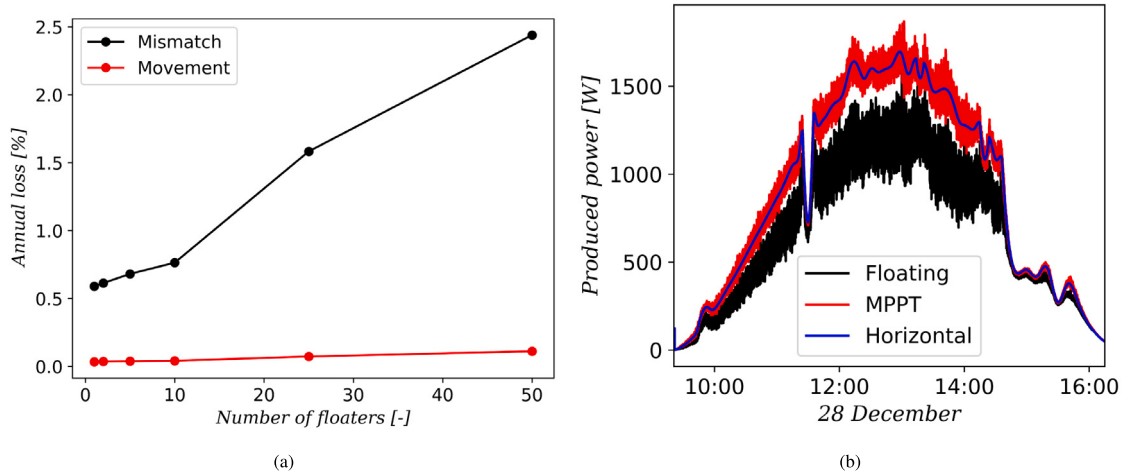
Fig. 12. (a) Plot of the yearly mismatch and movement losses of PLS systems for an increasing number of floaters. (b) Plot of the power produced by the floating, MPPT, and horizontal PLS-NF25 systems on the day with the highest mismatch losses.
