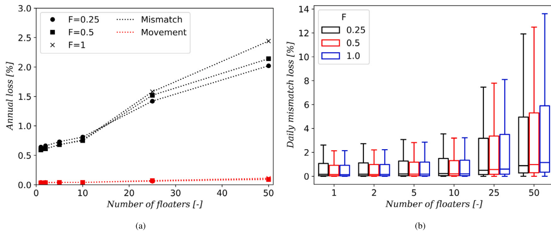
Fig. 19. (a) Plot of annual power losses and (b) boxplots of the daily mismatch for systems with varying fill factors for an increasing number of floaters.
