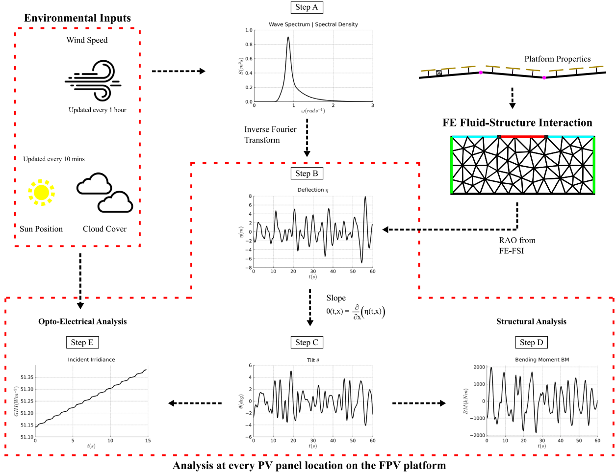
Fig. 2. Schematic of the solution procedure for the multi-physics problem.
