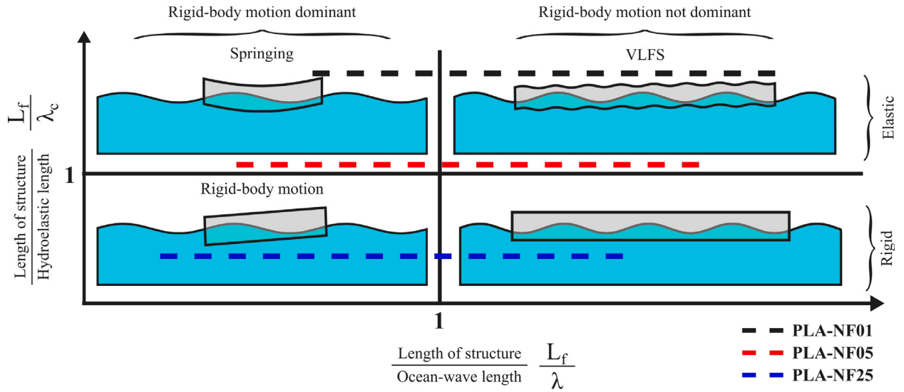
Fig. 9. Classification of the global response of floating structures [44]. The lines indicate the regime for PLA-NF01, PLA-NF05 and PLA-NF25.
