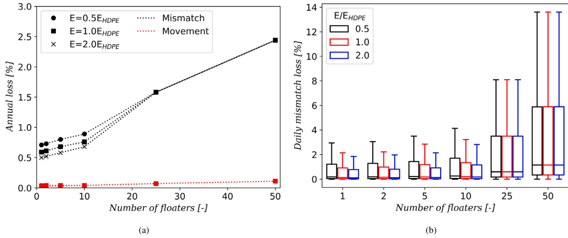
Fig. 16. (a) Plot of annual power losses and (b) boxplots of the daily mismatch for systems with varying Young's modulus for an increasing number of floaters.
