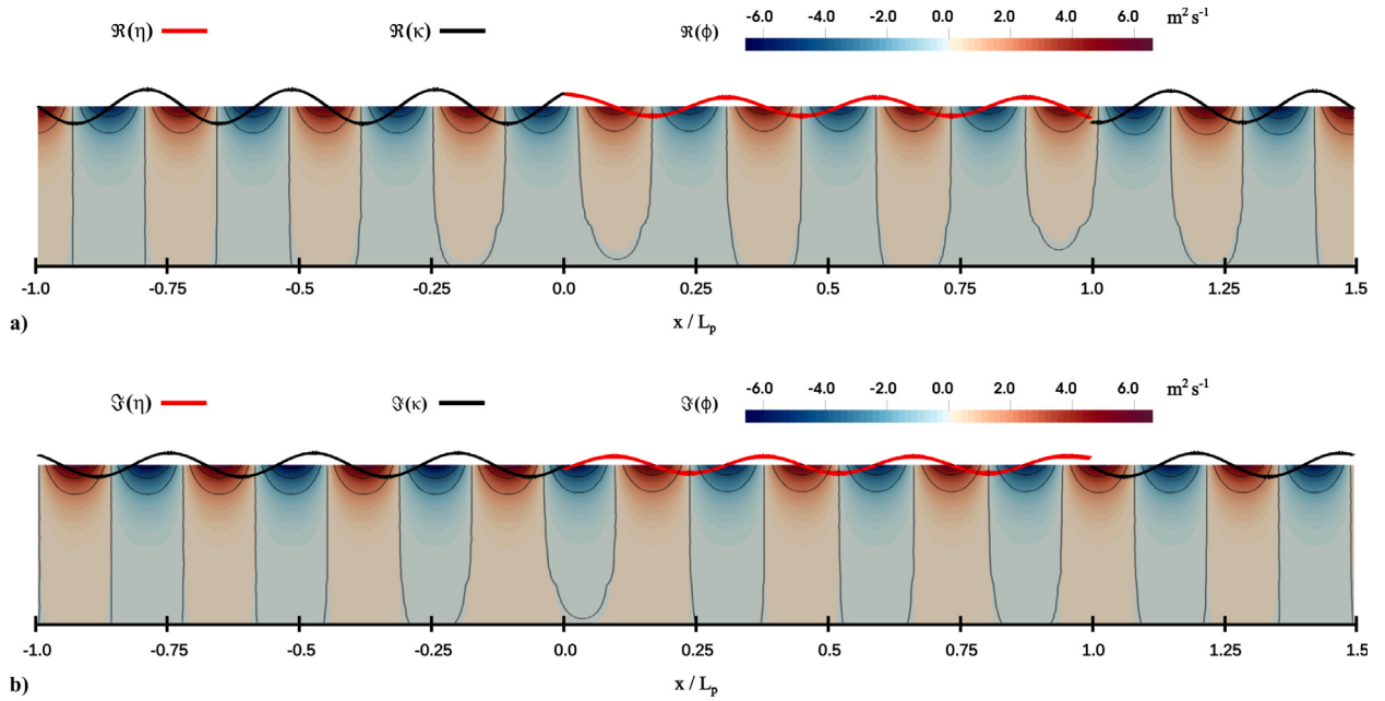
Fig. 4. Contour plot of \phi and line plots of \kappa and \eta , obtained from the FE-FSI model, due to the interaction of PLA-NF01 platform with ocean wave of frequency \omega = 1.5 \text{ rad s}^{-1} . (a) Real values of the solution. (b) Imaginary values of the solution.
