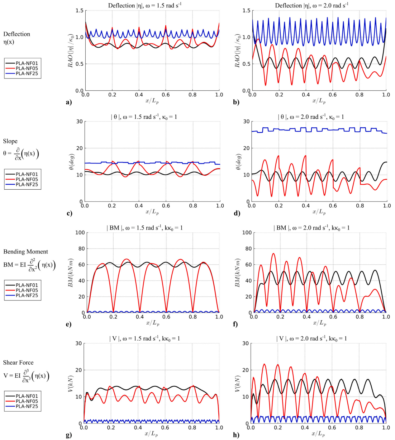
Fig. 5. Plots of the structural response of PLA-NF01, PLA-NF05 and PLA-NF25 floating platforms to monochromatic ocean-wave excitation of \omega = 1.5 \text{ rad s}^{-1} and \omega = 2.0 \text{ rad s}^{-1} . (a–b) Magnitude of beam deflection and (c–d) magnitude of tilt, along the length of the platform. (e–f) Magnitude of bending moment (BM) and (g–h) magnitude of shear force in the cross-section, per unit beam-width for unit-slope wave excitation.
