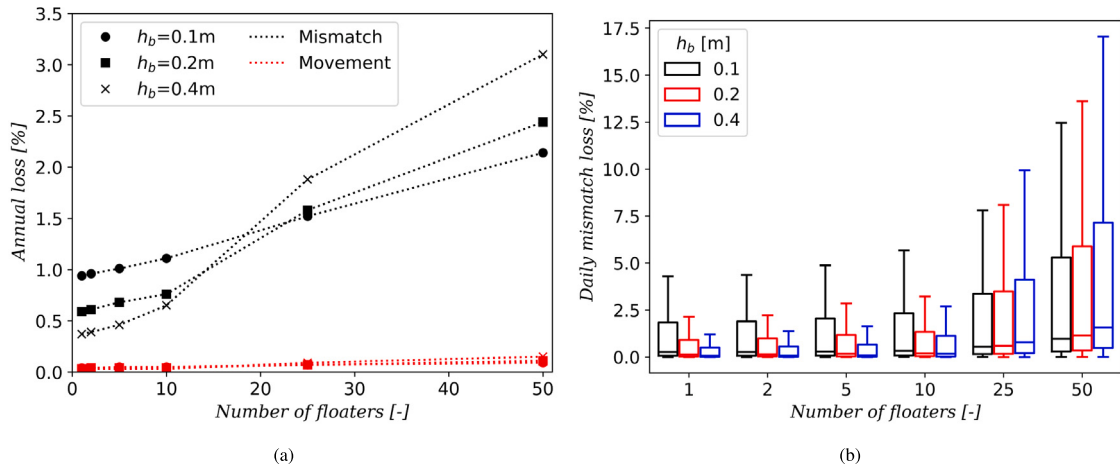
Fig. 17. (a) Plot of annual power losses and (b) boxplots of the daily mismatch for systems with varying thicknesses for an increasing number of floaters.
