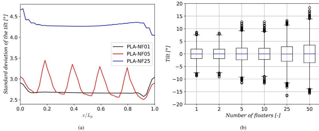
Fig. 11. (a) Plot of the standard deviation of the tilt along the platform for PLA-NF01, PLA-NF05, and PLA-NF25. (b) Boxplot of the tilt values over time at x = 0.19 \cdot L_p for an increasing number of floaters. Both figures considered the tilt from 9:00 to 10:00 on 1 January.
