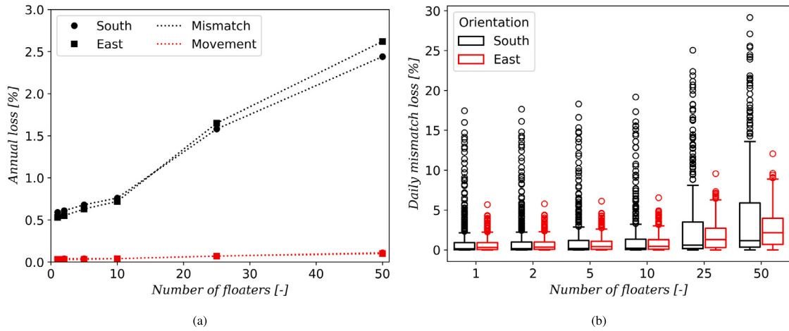
Fig. 14. (a) Plot of annual power losses and (b) boxplots of the daily mismatch for the systems facing South (PLS) and East (PLE) for an increasing number of floaters.
