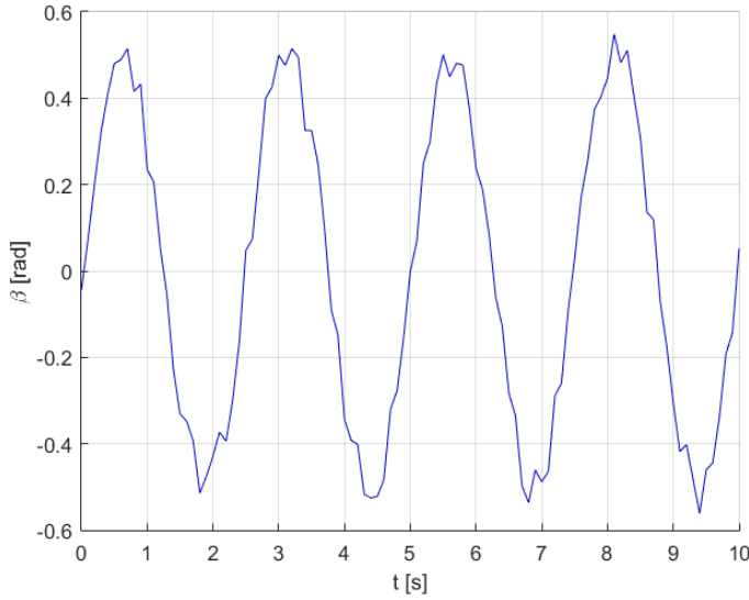
Figure 4.4: The first ten seconds of input \beta(t) provided to the pitch-plunge system during its identification through the SONIG algorithm. It is a sinusoid with distortions added for extra excitations.
