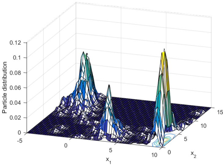
Figure 6.6: The probability distribution of the maximum of the GP approximating the Branin function, after generating measurements according to Thompson sampling. The three optima have been identified, some stray particles still reside in the lesser explored regions, and no particles remain in the part of the input space that has been explored but was found suboptimal.
