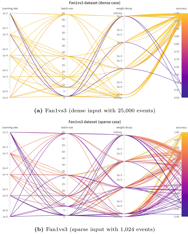
Fig. 2. Parallel coordinate plots showing HP tuning results for Fan1vs3 dataset using dense and sparse inputs. HPs: learning rate, batch size, and weight decay. In the dense setting, we observe test accuracies concentrated near the maximum accuracy, while in the sparse setting, we observe a small number of runs achieving the maximum accuracy. The plots are from the Weight and Biases website [4].
