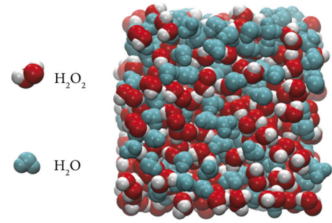
Fig. 1. A snapshot of a simulation box containing 250 \text{H}_2\text{O}_2 (red and white spheres represent oxygen and hydrogen atoms, respectively) and 250 \text{H}_2\text{O} molecules (green spheres), generated by the Visual Molecular Dynamic (VMD) software [95].
