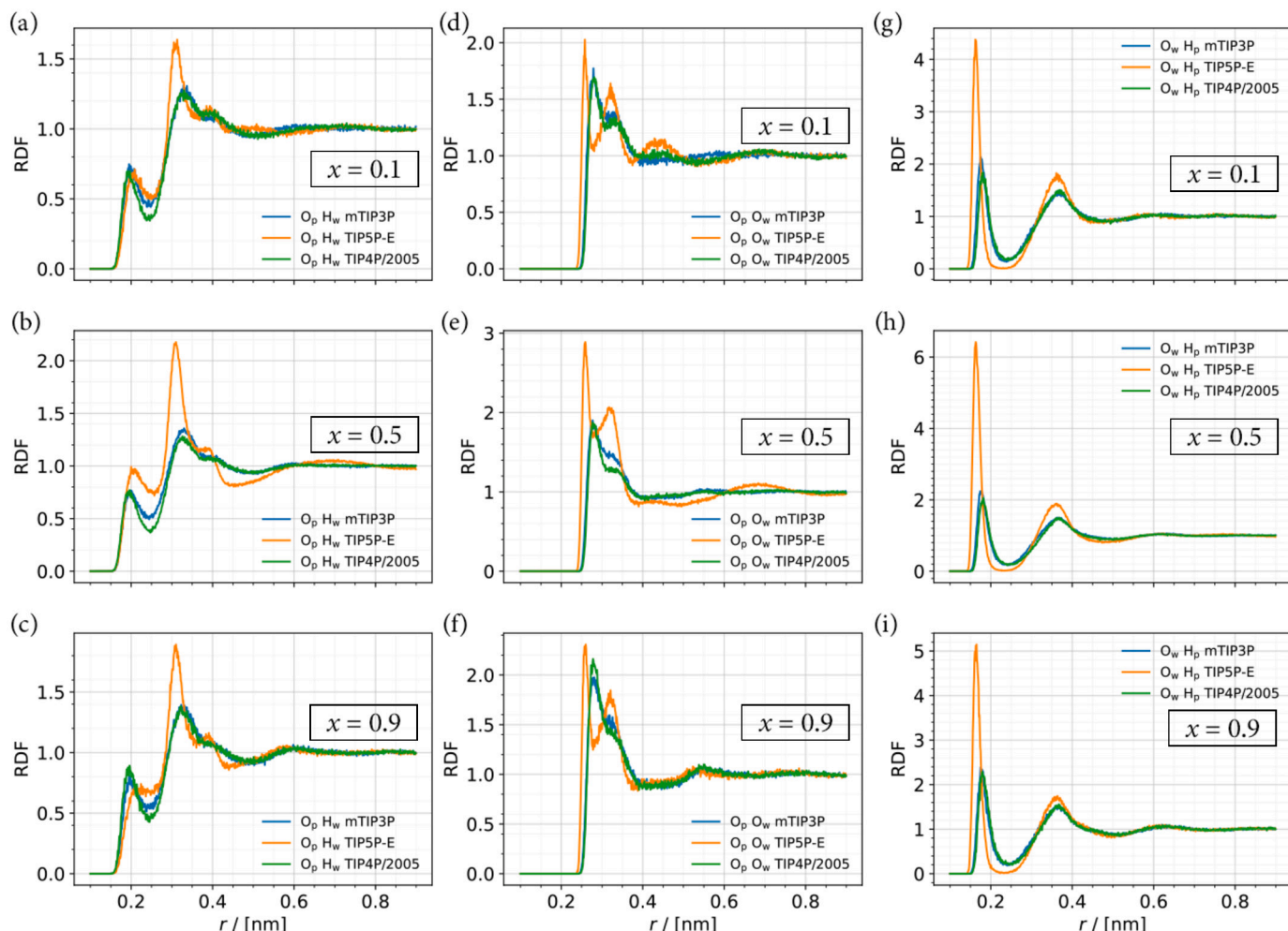
Fig. 8. Radial distribution functions (RDFs) as a function of radial distance, r [nm], for O_p (O of H_2O_2 ) and H_w (H of water) (a - c), O_w (O of H_2O_2 ) (d - f), and O_w (O of water) and H_p (H of H_2O_2 ) (g - i) for systems using the mTIP3P [68], TIP5P-E [77,84], and TIP4P/2005 [75] water force fields in combination with the Orabi force field for x = 0.1 , x = 0.5 , and x = 0.9 at 298 K and 1 bar, where x is the mole fraction of H_2O_2 .
