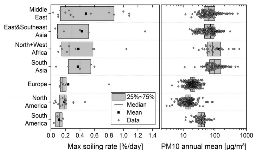
Figure 2. Maximum Daily Soiling Rates vs. Annual Mean Airborne Dust Concentrations of PM_{10} Across Various Regions.
