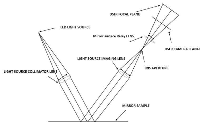
Figure 5. Optical Layout of the DSLR-Based Contamination Camera.
