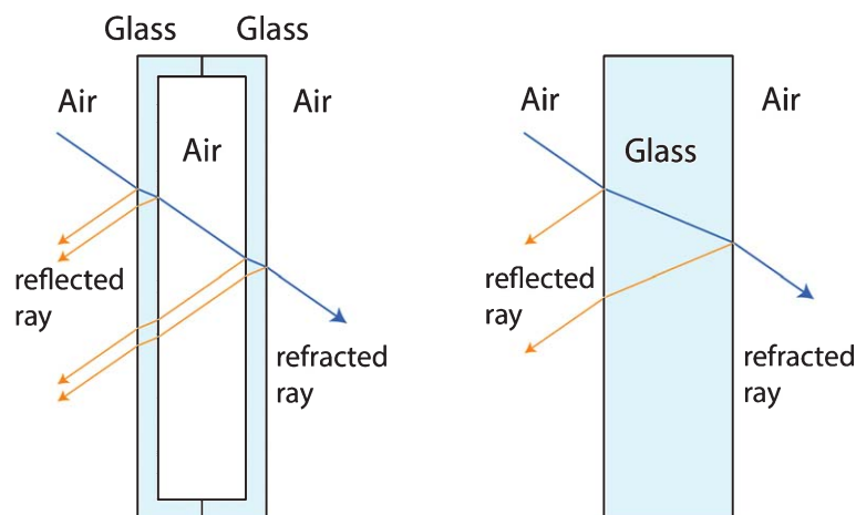
Fig. 1. The transition of the light rays through multiple media in a hollow glass block results in much more distortion compared to a solid glass block.
