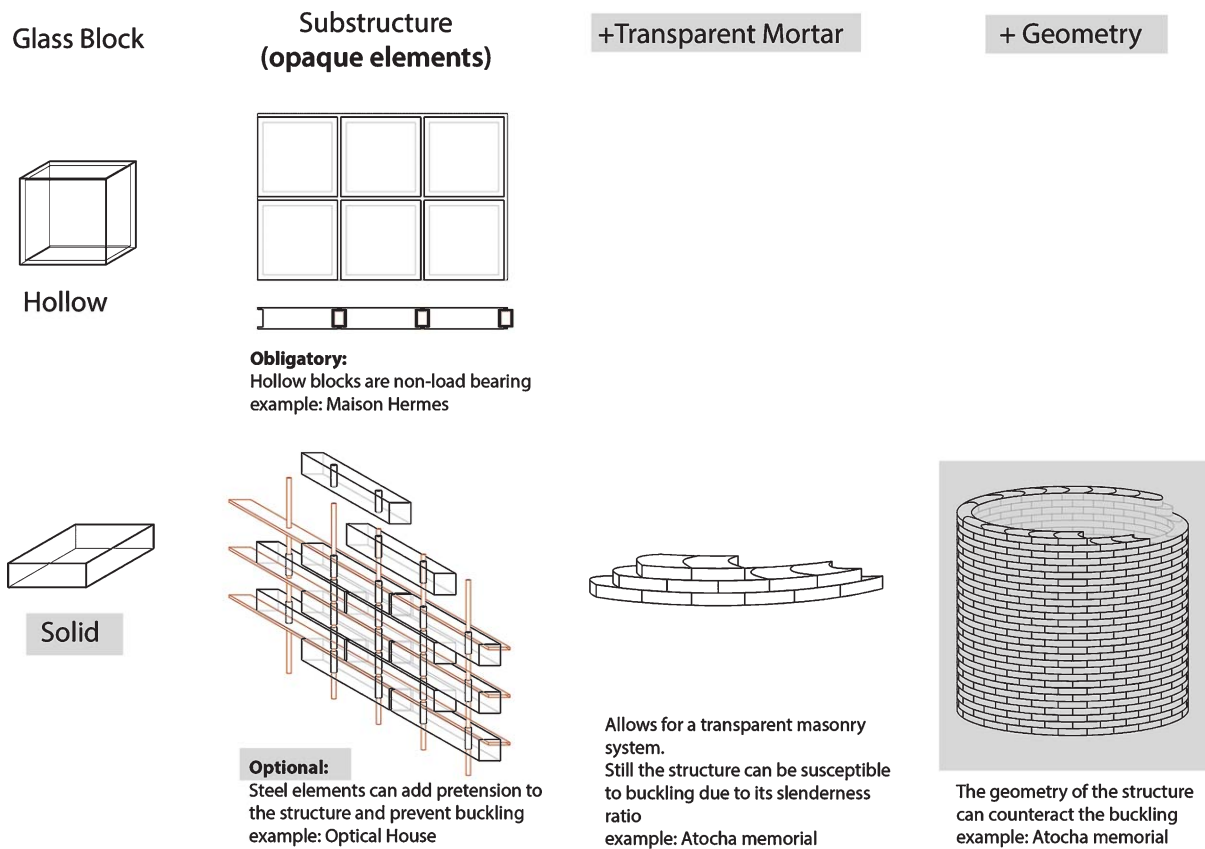
Fig. 2. Prerequisites for a completely transparent, structurally efficient glass block facade.
