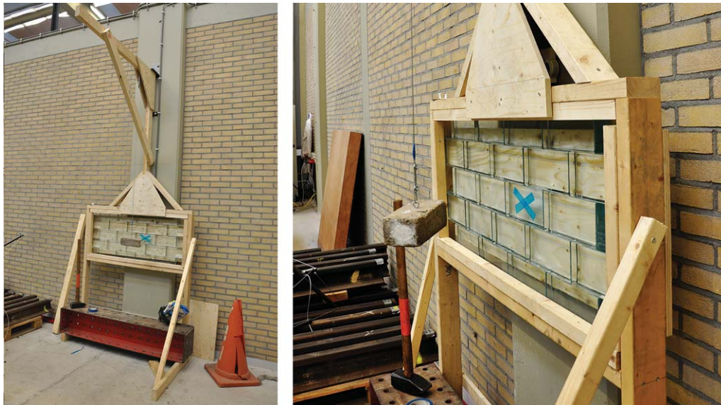
Fig. 10. Impact and vandalism test set-up.
