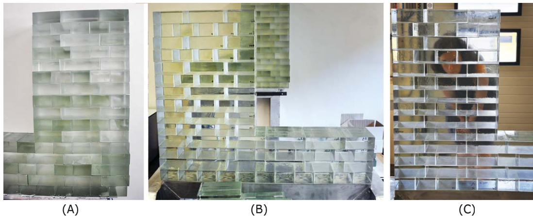
Fig. 7. Photographs of the three mock-ups. The first mock-up (A) was made with larger tolerances. As a result there were significant offsets in both height and width and also open joints between blocks. Centre: Mock-up (B). Higher accuracy in the size of the blocks counteracted the offset. Nevertheless, an unevenness of up to \pm 0.5 mm in flatness resulted in cavities and bubbles in the bond layer. Right: Mock up (C). All blocks meet the \pm 0.25 mm tolerance, resulting in an even spread and thus homogeneous bonding with an optimum visual result with no cavities or bubbles.
