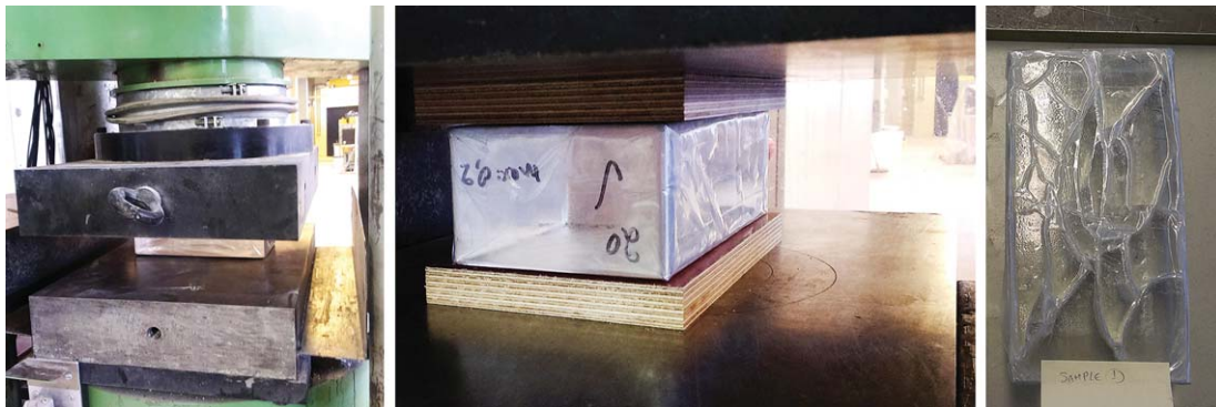
Fig. 12. Compression tests of glass blocks. Left: Test set-up for the two first series of blocks. Middle: Test set-up for the last series of blocks. Right: Typical initial crack pattern in specimen.
