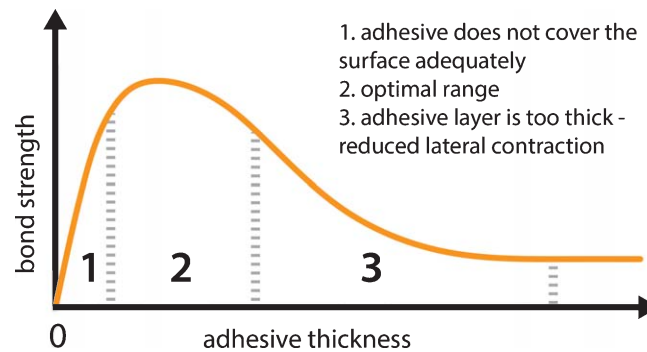
Fig. 4. Schematic Illustration of the relation between the optimum strength and the thickness of adhesive (Den Ouden, 2009; Riewoldt, 2014).
