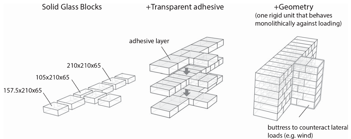
Fig. 5. Basic structural scheme of the proposed system.
