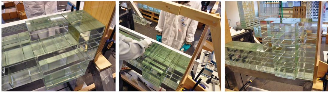
Fig. 8. Photographs of the final mock-up which includes the buttress's construction by interlocking glass blocks.
