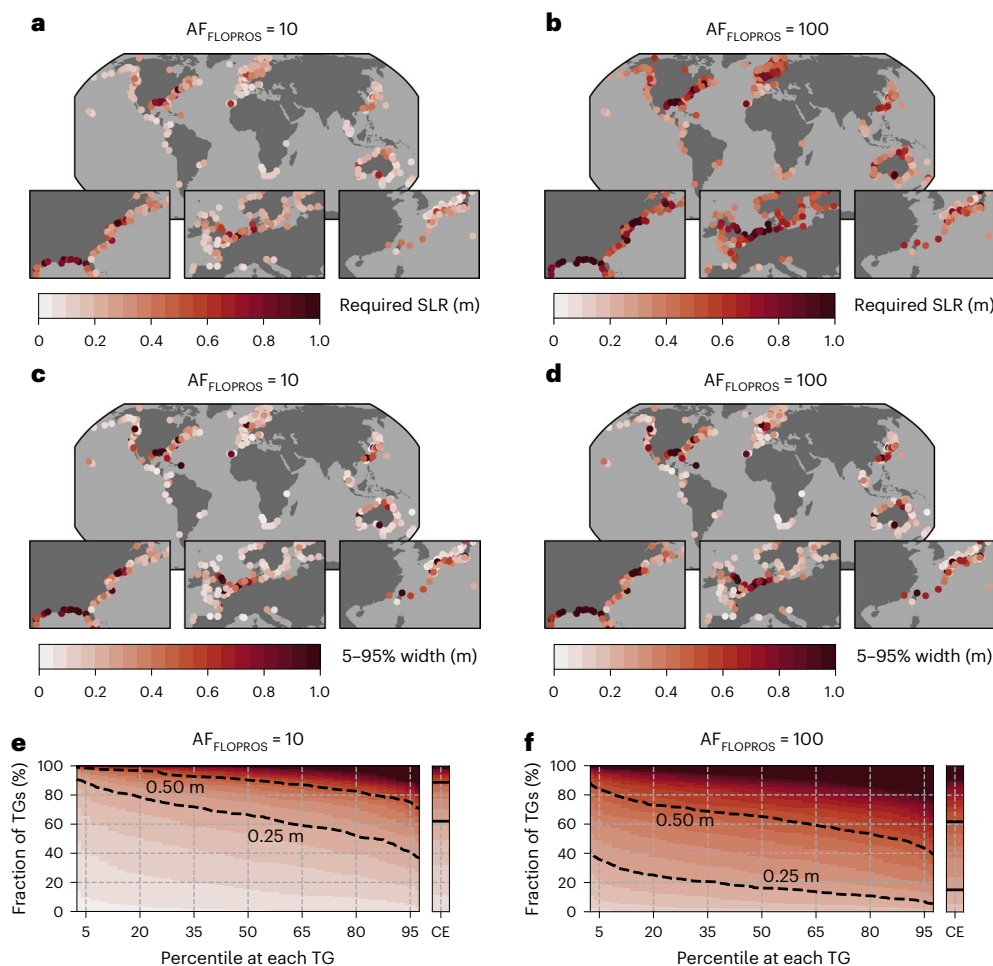
Fig. 3 | Required SLR for \text{AF}_{\text{FLOPROS}} = 10 and 100 . a, b , Central estimate of required SLR (m) for \text{AF}_{\text{FLOPROS}} = 10 ( a ) and 100 ( b ) at GESLA3 tide gauges. c, d , Width of the 5–95% range of required SLR (m) for \text{AF}_{\text{FLOPROS}} = 10 ( c ) and 100 ( d ). e, f , Fraction of tide gauges (TGs) requiring the displayed amount of SLR (m) or less for \text{AF}_{\text{FLOPROS}} = 10 ( e ) and 100 ( f ), for different percentiles at each TG (left) and
