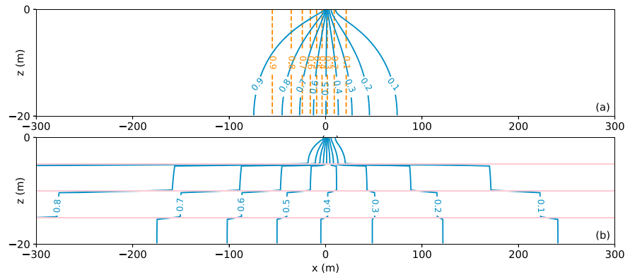
Figure 4. (a) Contours of the relative amplitude in a homogeneous unconfined aquifer for a tidal period of \tau = 0.5 d. Single-layer model (red dash) and 80-layer model (blue). (b) Contours of the relative amplitude when three thin clay layers of 25 cm (pink) are present in the aquifer.
