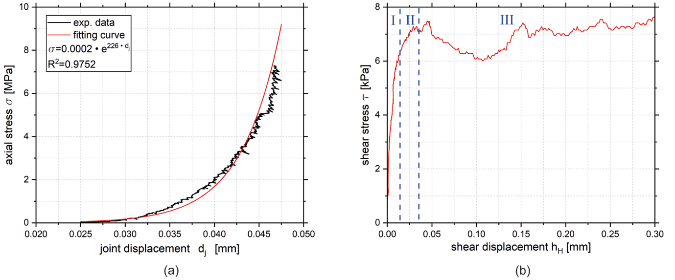
Fig. 2. (a) Fitting process to evaluate the stress dependency of joint normal stiffness and (b) example of the stress-displacement curve obtained from direct shear tests.
