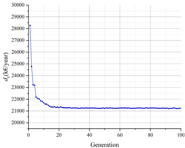
Fig. 9. Convergence of the optimisation results with the increase of the generation.
