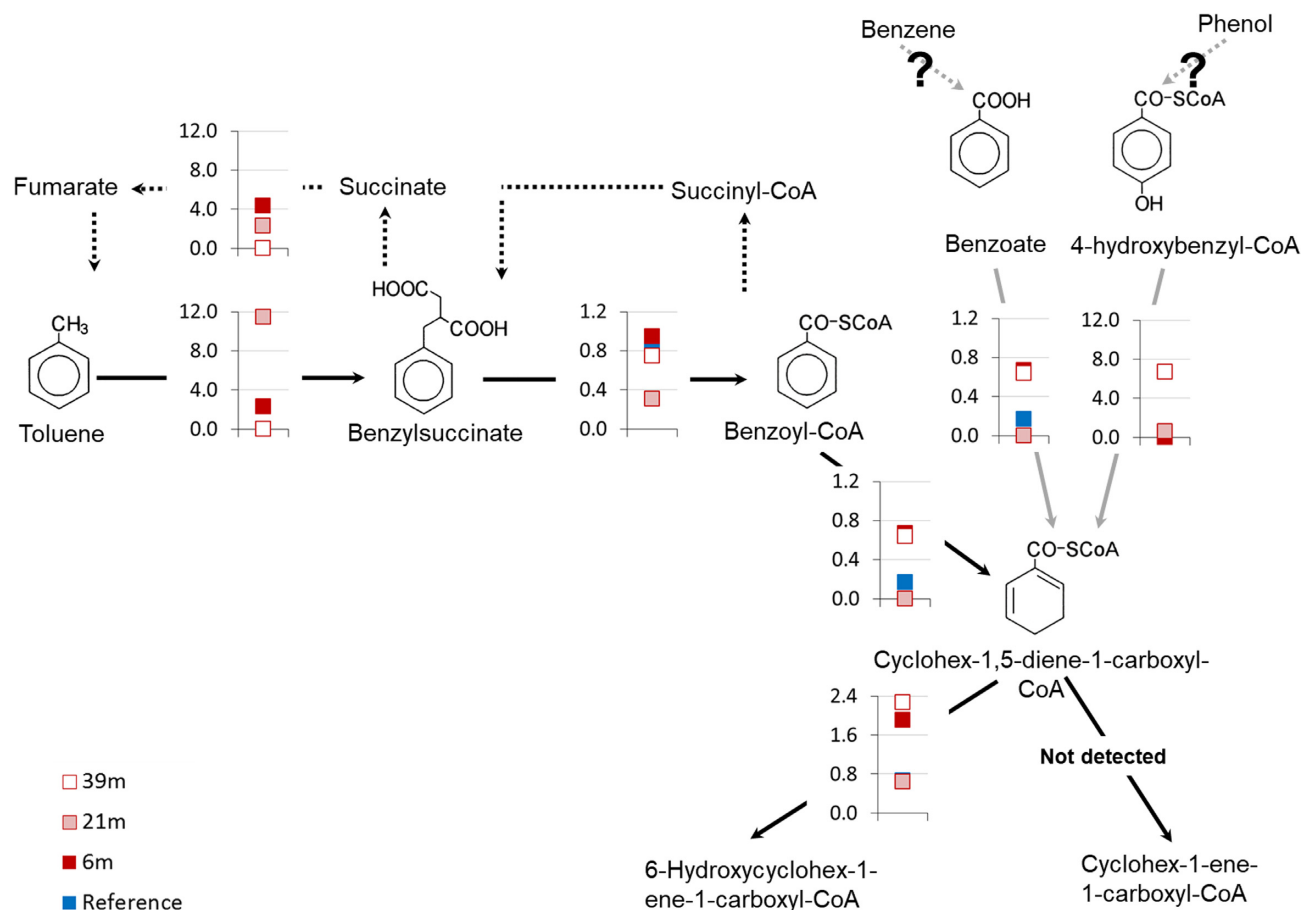
Figure 3. Expression levels (relative transcriptional activity; y-axis) of genes belonging to toluene, benzoate and 4-hydroxybenzyl-CoA degradation pathways. Expression of the key genes converting toluene to benzylsuccinate (benzylsuccinate synthase, bs ) was detected only at 6 m and 21 m downstream of the landfill. Benzoyl-CoA reductase involved in the degradation of benzoyl-CoA to cyclohex-1,5-diene-1-carboxyl-CoA were found in all MGs and had relatively high expression levels in contaminated wells.
