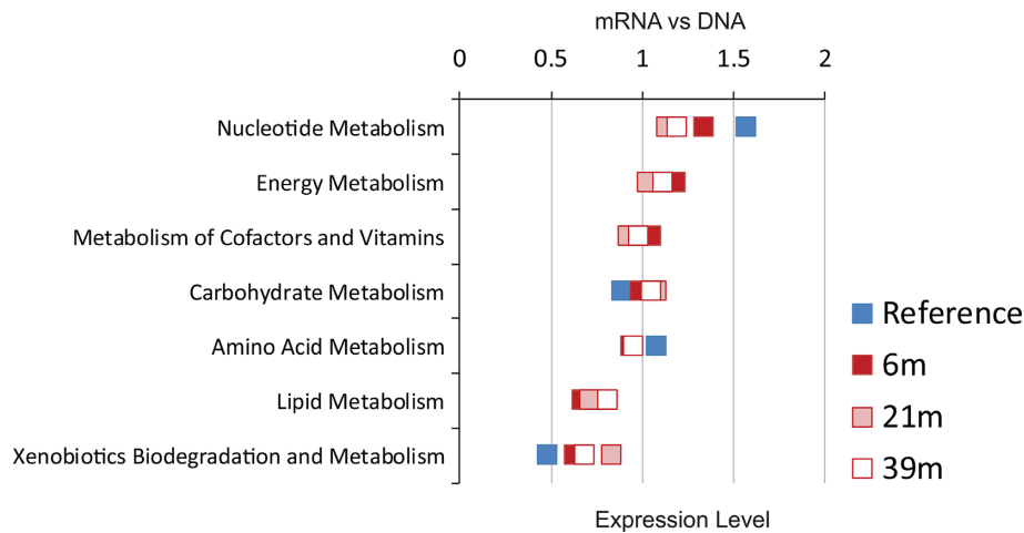
Figure 2. Differences in expression levels (relative transcriptional activity) of KEGG metabolism classifications among sampling wells. Expression levels were calculated in Equation (2) for each well.
