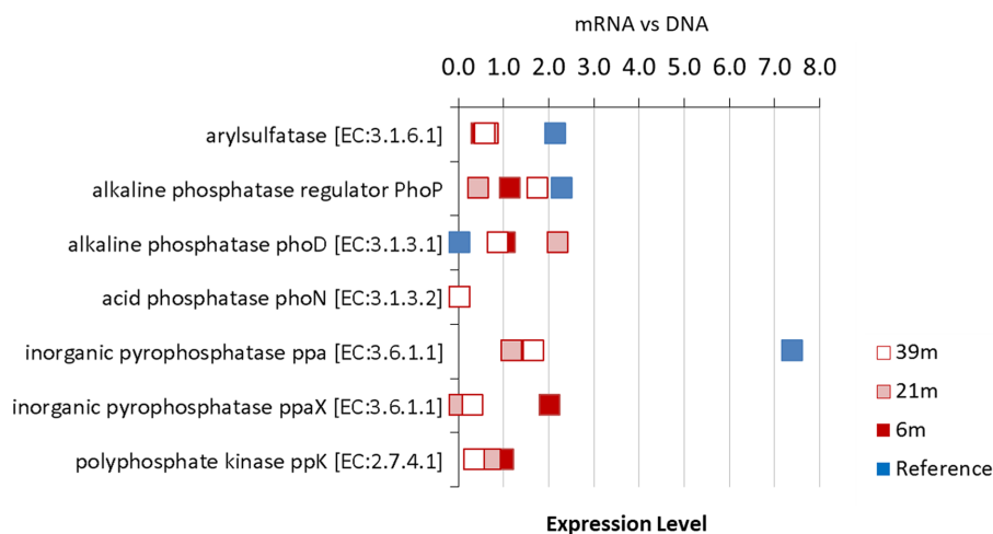
Figure 5. Expression levels (relative transcriptional activity) of several genes encoding for phosphate acquisition in Banisveld aquifer.
