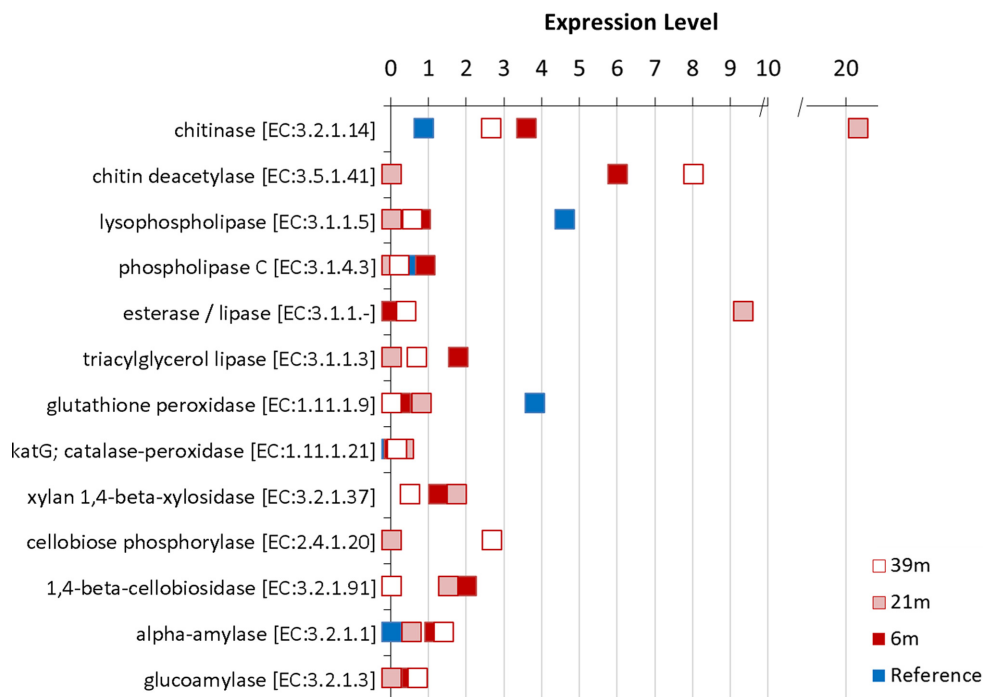
Figure 4. Expression levels (relative transcriptional activity) of several genes encoding carbon degradation such as chitinases and xylanases were higher in contaminated groundwater wells. Expression levels were calculated in Equation (2) for each well.
