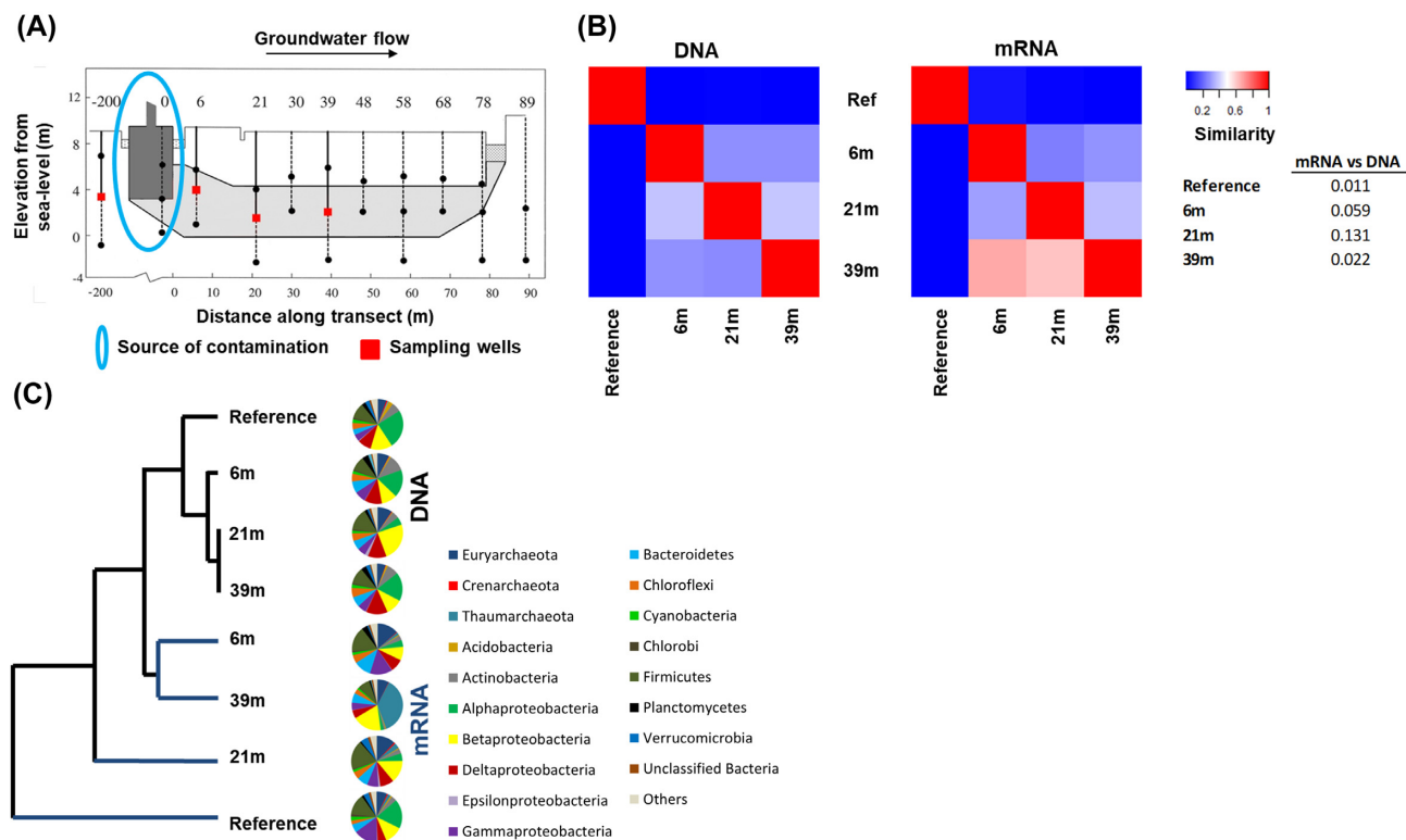
Figure 1. (A) Sampling locations along the aquifer polluted by the Banisveld landfill. Grey represents the shape of the plume and sampling wells are demonstrated in red. Groundwater sampling wells are indicated by their corresponding distance from the landfill. (B) Similarity matrix resulting from the comparison of MG and MT reads with Compareads between different samples from the Banisveld aquifer. Color levels correspond to similarity levels; red-high similarity, blue-low similarity (see scale: 0 dissimilar–1 similar). Based on both DNA and mRNA analyses, the reference was highly dissimilar to the contaminated wells. The table shows the similarity calculated between DNA and mRNA reads in each well. (C) Cluster analysis based on Euclidean distance and generated with the MEGAN software with the UPGMA algorithm for Banisveld MG and MT read annotations from BLASTX results. Pie charts show the phylogenetic distributions of the reads.
