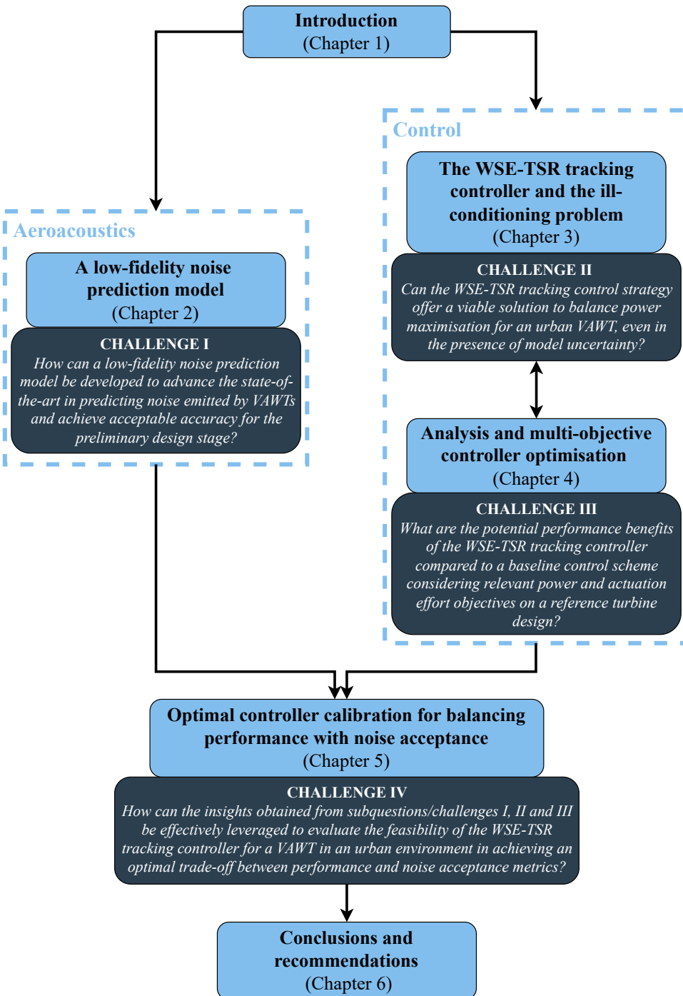
Figure 1.3: Thesis outline
