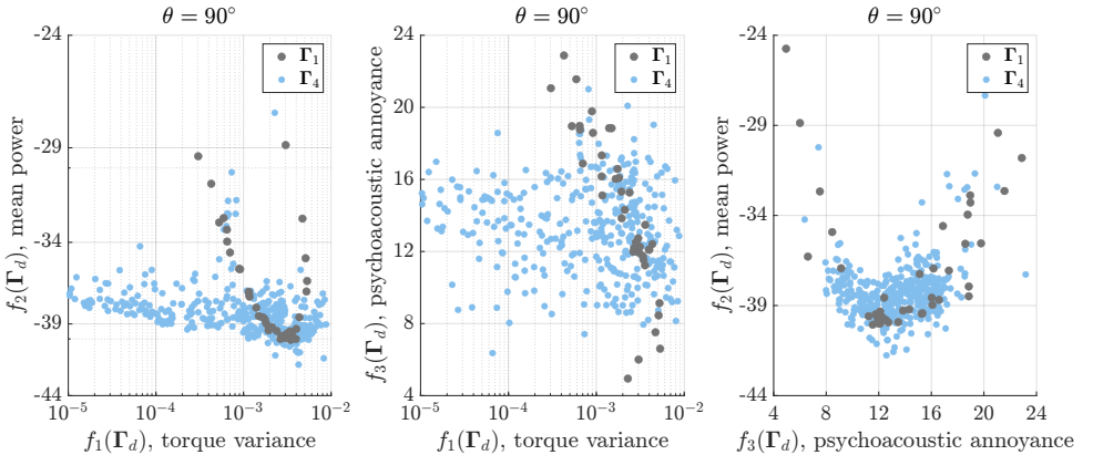
Figure 5.9: Results for the WSE-TSR tracking control scheme under realistic turbulent wind conditions obtained with an exploratory search of two estimator-controller design variables: \Gamma_1 and \Gamma_4 . The three objective functions \mathbf{f}(\Gamma_d) define the performance space for the controller. For the calculation of the psychoacoustic annoyance, the microphone in the x-z plane at \theta = 90^\circ is selected.
