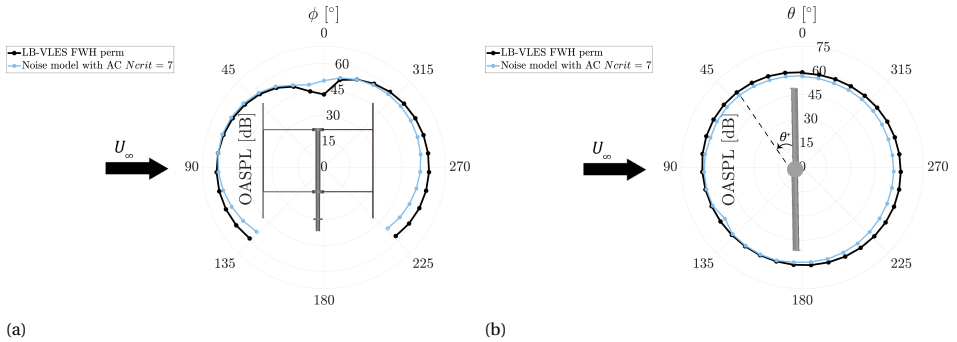
Figure 2.17: Directivity plots of the Overall Sound Pressure Level (OASPL) computed on: a circular array of 27 microphones in the x-y plane (Figure 2.17a) and on a circular array of 36 microphones in the x-z plane (Figure 2.17b). The LB-VLES results are compared with results from the noise model with AC data for N_{crit} = 7 .
