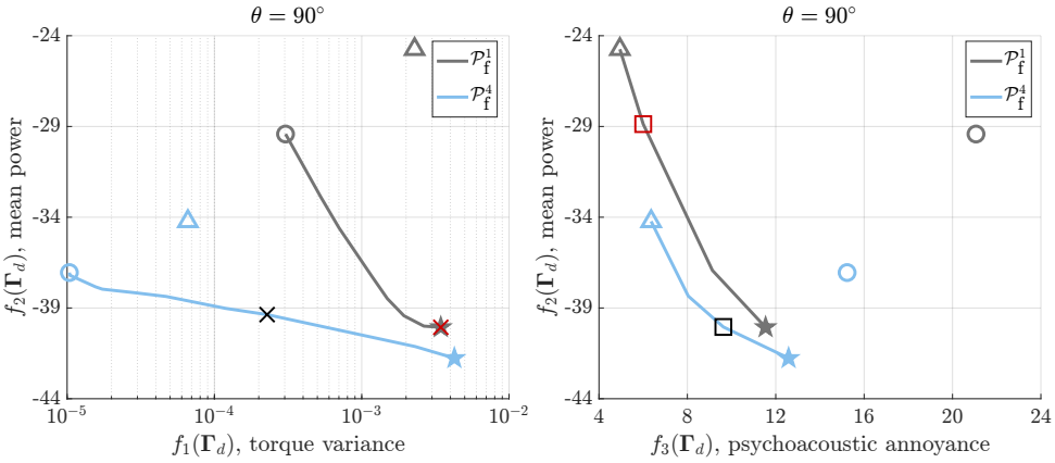
Figure 5.10: Pareto fronts \mathcal{P}_f^1 and \mathcal{P}_f^4 obtained for the K\omega^2 and the WSE-TSR tracking control schemes under realistic turbulent wind conditions, respectively. For the calculation of the psychoacoustic annoyance, the microphone \theta = 90^\circ is selected in the x-z plane. The optimal solutions for f_1(\Gamma_d) , f_2(\Gamma_d) and f_3(\Gamma_d) are indicated using circles (○), stars (☆) and triangles (Δ), respectively. The trade-off solutions for the two controllers are shown with a cross (x) when f_1(\Gamma_d) and f_2(\Gamma_d) are considered as objectives, and with a square (□) when f_2(\Gamma_d) and f_3(\Gamma_d) are considered. In contrast to the baseline controller, the WSE-TSR tracking controller achieves improved power maximisation while reducing torque fluctuations and psychoacoustic annoyance, albeit with a slight compromise in power extraction.
