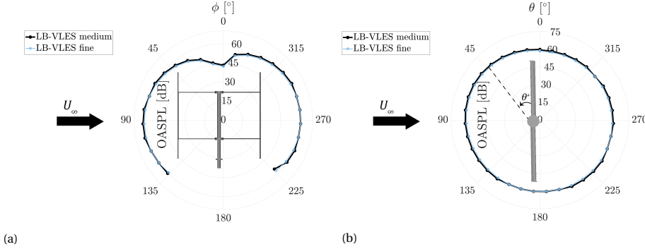
Figure 2.9: Directivity plots of the Overall Sound Pressure Level (OASPL) computed on: a circular array of 27 microphones in the x-y plane (Figure 2.9a) and on a circular array of 36 microphones in the x-z plane (Figure 2.9b). The LB-VLES results with the medium resolution are compared with the LB-VLES results with fine resolution.
