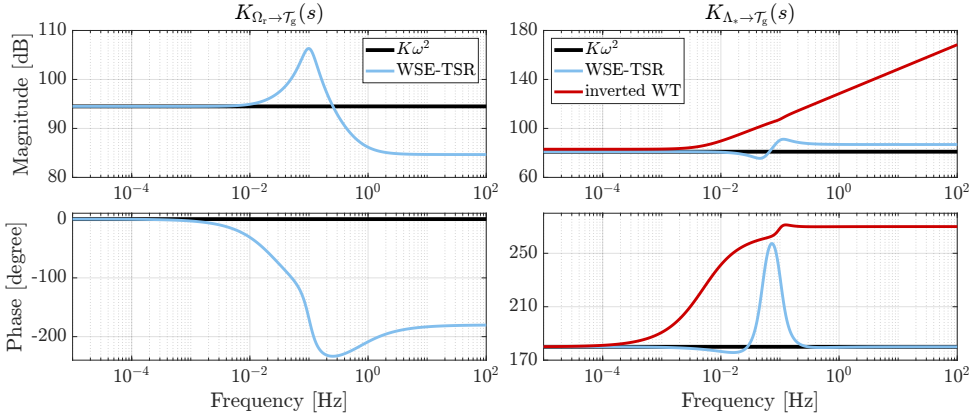
Figure 4.6: Bode plots of the controller transfer functions K_{\Omega_r \rightarrow \mathcal{T}_g}(s) and K_{\Lambda_* \rightarrow \mathcal{T}_g}(s) for the K\omega^2 controller ( black line) and the WSE-TSR tracking controller ( cyan line) without optimal calibration. For the baseline, both transfer functions are frequency-independent. For the combined scheme, in the low-frequency region, K_{\Omega_r \rightarrow \mathcal{T}_g}(s) and K_{\Lambda_* \rightarrow \mathcal{T}_g}(s) have gains equal to the baseline. In particular, for the right-hand plot, the controller gains match the inverted model of the wind turbine ( red line), exhibiting a second-order lead-lag behaviour. By contrast, for higher frequencies, the response varies for both transfer functions for the combined scheme.
