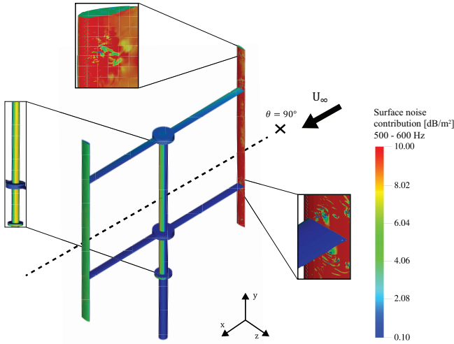
Figure 2.23: FWH integral contribution from a microphone in the x-z plane at \theta = 90^\circ .
