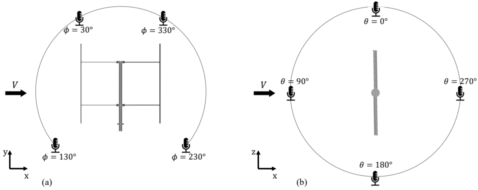
Figure 5.7: Two circular arrays of virtual microphones are positioned at a distance of 2.6D from the centre of the VAWT. Array (a) comprises 4 microphones located in the x-y plane, while array (b) consists of 4 microphones positioned in the x-z plane. These locations are considered relevant for characterising the psychoacoustic annoyance of the sound source.
