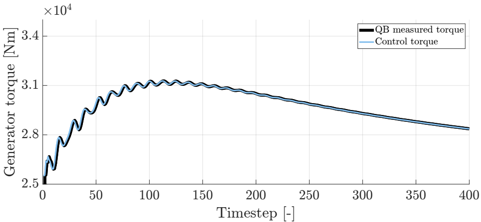
Figure D.2: Output of the example code running the K\omega^2 controller.
