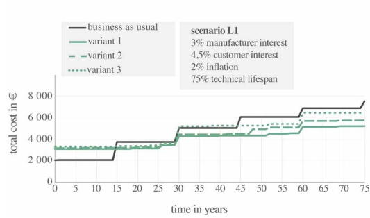
FIG. 2.6 Comparison scenario L1 of total costs for three CIK variants and the business-as-usual case.
