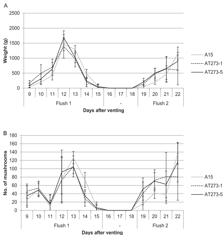
Figure 3.2: Average biomass (a) and number of mushrooms (b) of A15, AT273-1 and AT273-5 mushrooms per box ( n=10 ) picked during a 22-day period after venting ( t = 0 ). Bars represent standard deviation.
