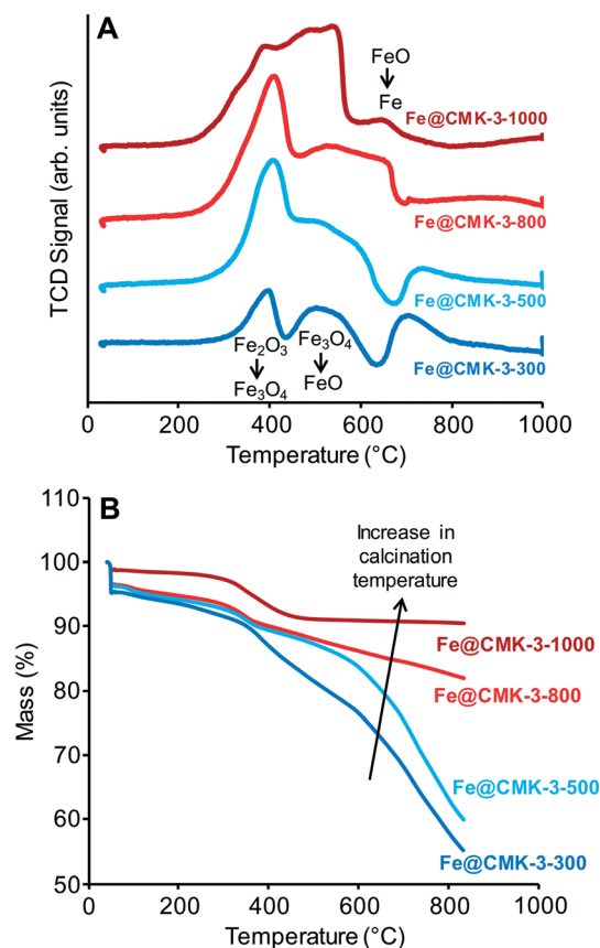
Fig. 3 (A) \text{H}_2 -TPR and (B) \text{H}_2 -TGA curves of the calcined Fe@CMK-3-300 (dark blue), Fe@CMK-3-500 (light blue), Fe@CMK-3-800 (light red), and Fe@CMK-3-1000 (dark red) catalysts.
