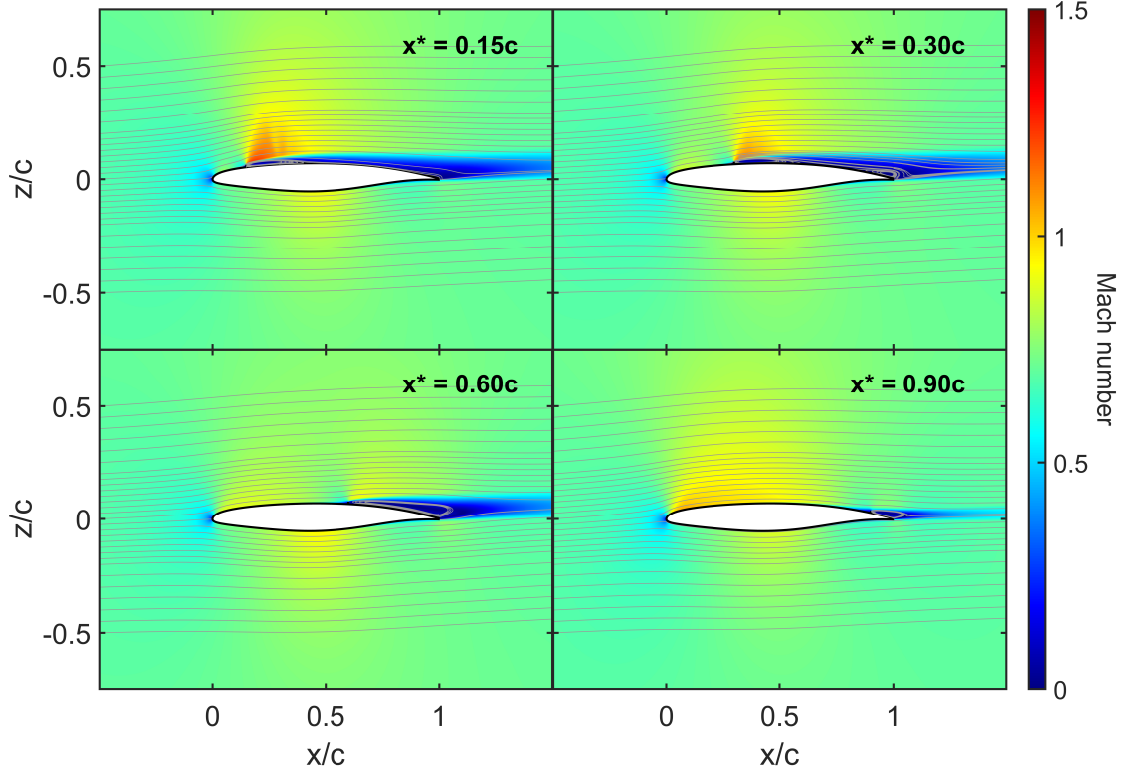
Fig. 10 Contour plot of the velocity field around the DLR-F25 wing section at y/b = 0.85 , with a mini-tab of height h/c = 0.02 positioned on the upper surface at different chord-wise locations, for M_\infty = 0.714 , Re_\infty = 6.93 \cdot 10^6 and \alpha = 2.15 deg.
