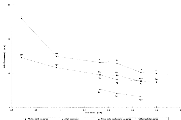
FIG. 7. Exchange core polarization (ECP) contributions to the hyperfine field in the alkaline-earth-metal-ion, alkali-metal-atom, group-IIB-ion and noble-metal-atom series, as fractions of valence contributions. Ionic radii used refer to the positive alkali-metal ions, as explained in the text.
