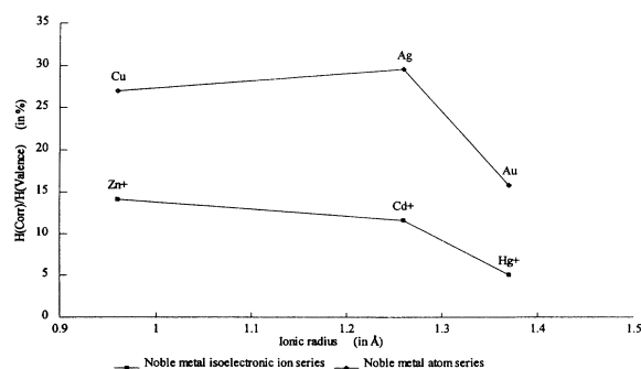
FIG. 9. Many-body correlation contribution to the hyperfine field in the group-IIB-ion and noble-metal-atom series. Ionic radii used refer to the appropriate positive alkali-metal ions, as explained in the text.
