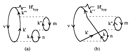
FIG. 6. Major third-order correlation diagrams. (0,3) diagrams representing (a) direct and (b) exchange correlation contributions to the hyperfine field.
