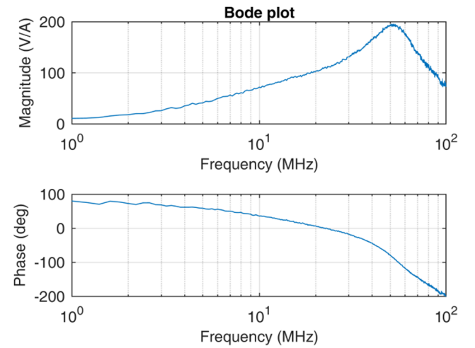
Fig. 7. Bode diagram of the magnetic loop antenna.
