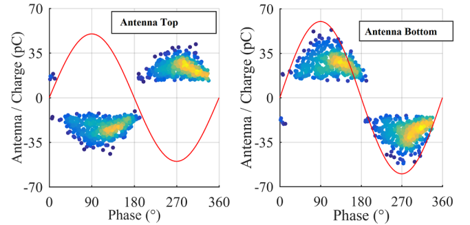
Fig. 17. PRPD of free moving particle test measured by left: top antenna, right: bottom antenna.
