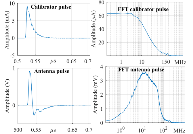
Fig. 6. Magnetic antenna response to a calibrator pulse.
