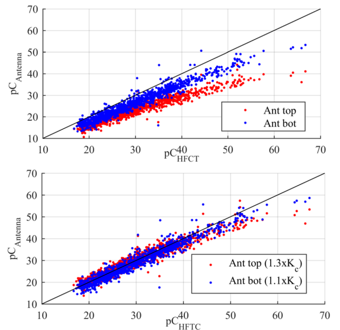
Fig. 18. Top: correlation between the charge values from the test cell HFCT and the antennas; bottom: compensation of the calibration factor.
