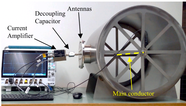
Fig. 5. Calibration rig workbench.
