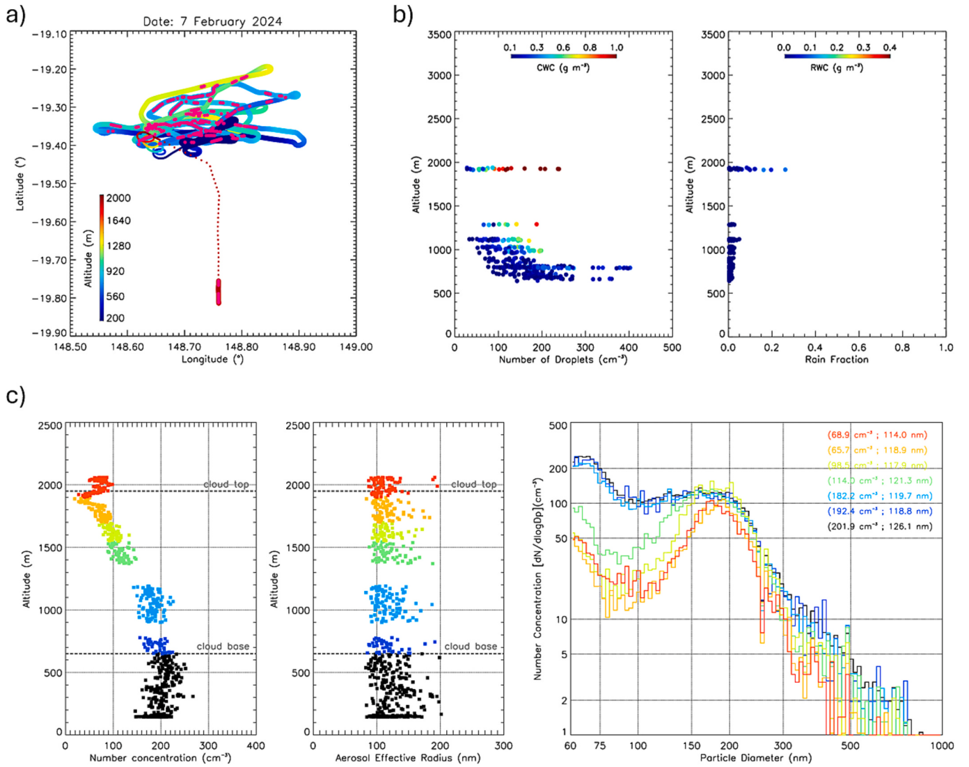
Fig. 8. a–c. Similar to Fig. 7a–c for measurements on 7 February 2024. The prevailing wind directions at 500 m, 1500 m, and 3000 m were S-SW, SE, and SE, respectively.
