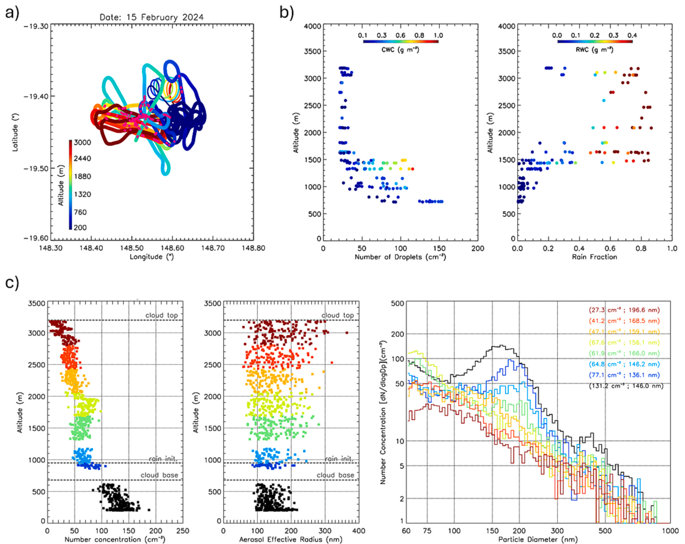
Fig. 9. a–c. Similar to Fig. 7a–c for measurements on 15 February 2024. The prevailing wind directions at 500 m, 1500 m, and 3000 m were E–SE, E–NE, and N–NE, respectively.
