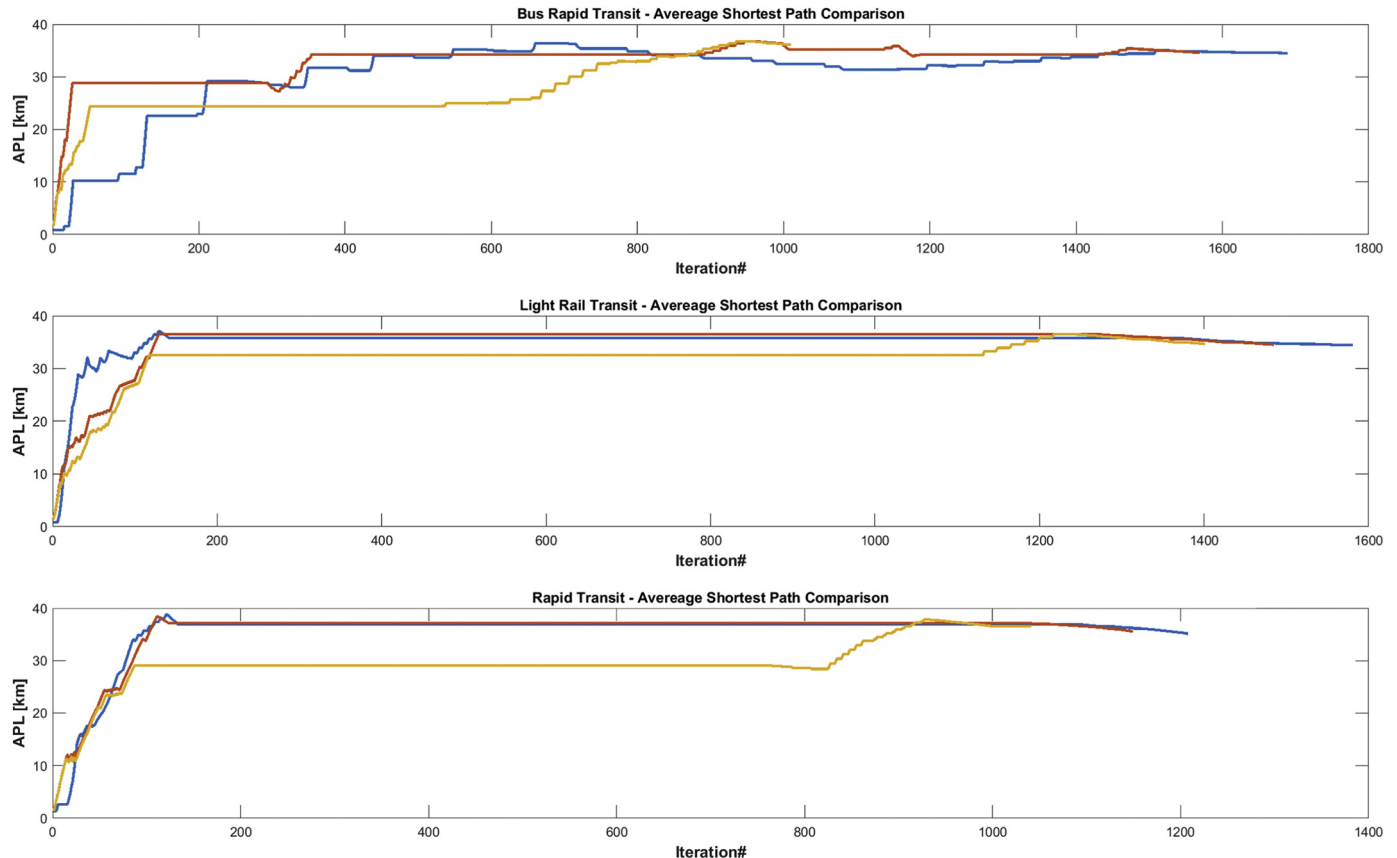
Fig. 3. Average shortest Path length (APL) for a given mode (BRT - top; LRT - middle; Metro - bottom) and varying population distributions (Uniform - blue; Linear - red; Exponential - orange). (For interpretation of the references to colour in this figure legend, the reader is referred to the web version of this article.)
