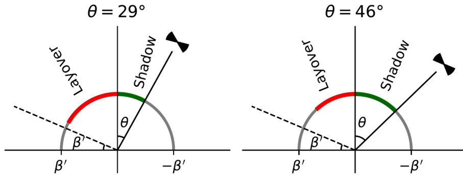
Fig. 4. 2D schematization of the effects of the surface geometry on the radar geometry. Illustrated are the minimum and maximum incidence angles \theta of Sentinel-1 for a variable, apparent slope \beta' \in [-90^\circ, 90^\circ] . Only the local effects, induced by the DEM-pixel itself, are described by these relations. Shadow or layover, induced by nearby topography, cf. Fig. 1 (b), cannot be captured this way.
