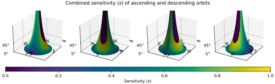
Fig. 8. A 3D interpretation of the results from Fig. 7. This image shows more clearly how shadow and layover affect only very steep slopes. Displacements along these slopes, as well as south facing, low relief slopes are less likely to be detectable. The ascending and descending orbit directions are shown in black at the bottom.
