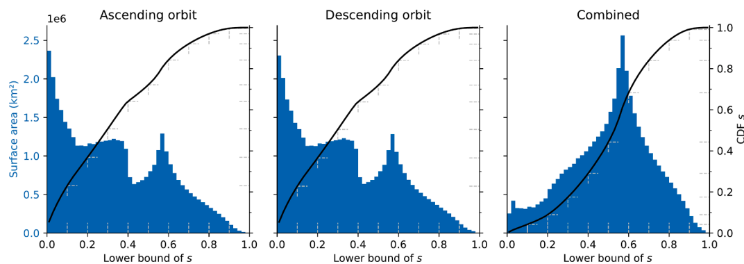
Fig. 11. Histograms of computed global sensitivity index values, for both ascending and descending orbits, as well as the highest sensitivity index from either orbit. Included are all slopes mapped by the Copernicus DEM, steeper than 5°. Areas invisible due to layover or shadow are marked as 0 sensitivity. The cumulative distribution function of the absolute value of the lower bound of sensitivity, is given in black.
