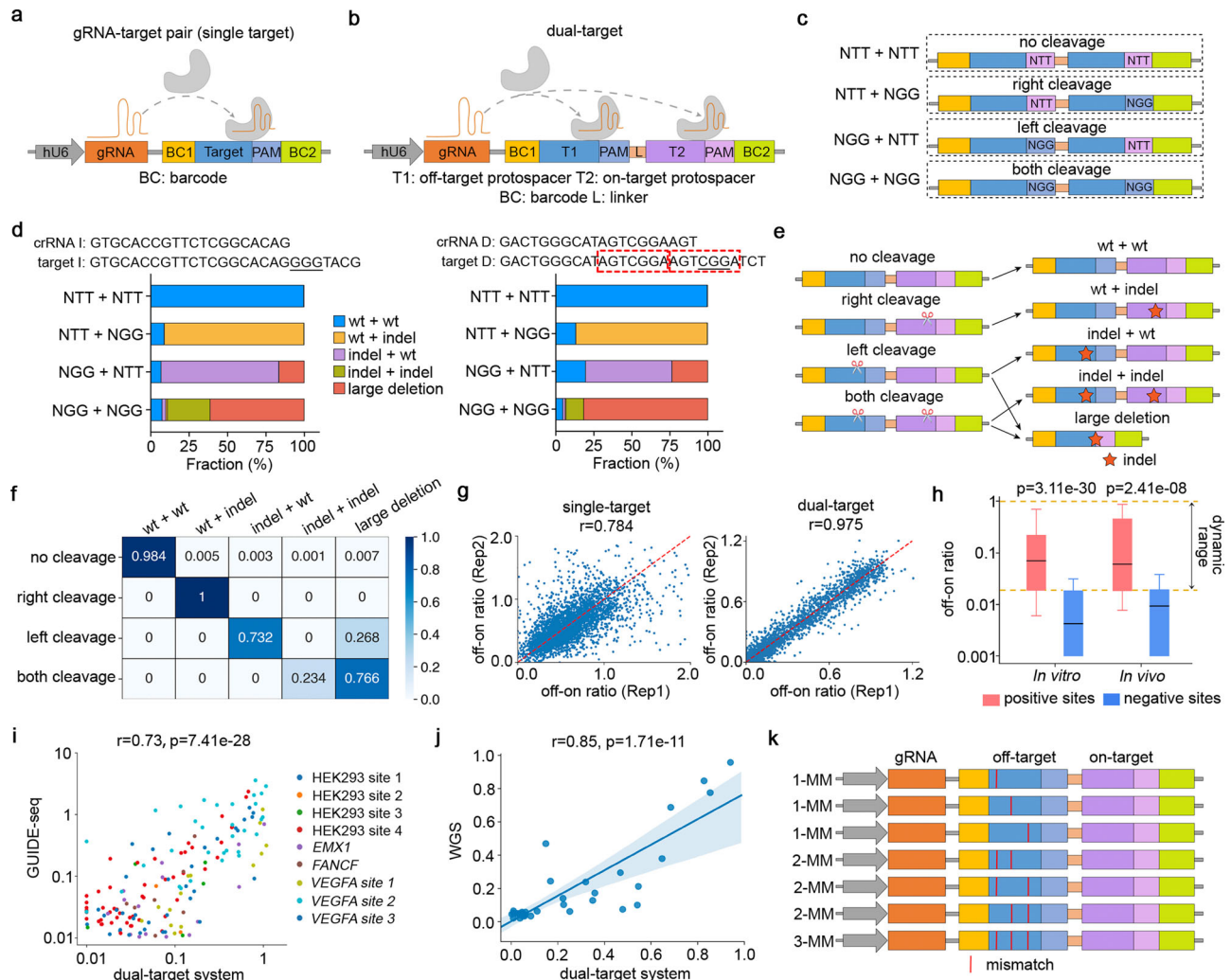
Fig. 1 Assessment of off-on ratios using a synthetic dual-target system. a, b A schematic representation of paired gRNA-target design using a single-target or b dual-target sequence. c The design of control dual-target sequences corresponding to 4 cleavage types, where the left and right protospacers are identical and the cleavage events are turned on or off by “NGG” or “NTT” PAM sequences, respectively. d Bar charts showing the fractions of five types of editing outcomes in relation to the 4 cleavage types. Left: a gRNA associated with dominating non-homologous end joining (NHEJ); right: a gRNA associated with dominating microhomology-mediated end joining (MMEJ), where the microhomology sequences are highlighted in red rectangles. e A demonstration of the cleavage-editing model of the dual-target system. f A heatmap showing the cleavage-editing transition matrix computed from mutational profiles of 276 control dual-target sequences. g Scatter plots showing the correlations of off-on ratios between biological replicates using single- or dual-target systems. h A box plot showing the distributions of the off-on ratios estimated by the dual-target system, corresponding to the 32 filtered benchmark gRNAs and 480 target sequences. Positive: reported off-target sequences; Negative: unreported genomic sequences with <5 mismatches relative to crRNA. The data represent n = 204 positive, 213 negative (in vitro), and n = 66 positive, 52 negative (in vivo) gRNA-target pairs. The box plot displays a median line, interquartile range boxes and min to max whiskers. The p -values were calculated using two-tailed Mann-Whitney U test. i, j Scatter plots showing the correlations between the off-on ratios estimated from the dual-target system and i GUIDE-seq or j WGS, at the reported genomic off-target sequences. The p -values were calculated using Pearson correlation test. The shadow represents the 95% confidence interval. k A demonstration of the off-target sequence design in the high-throughput experiments using the dual-target synthetic system, where the mismatches in the 2-MM and 3-MM sequences are the combinations of the mismatches in the 1-MM sequences. Source data for Fig. 1d, g–j are provided in the Source Data file.
