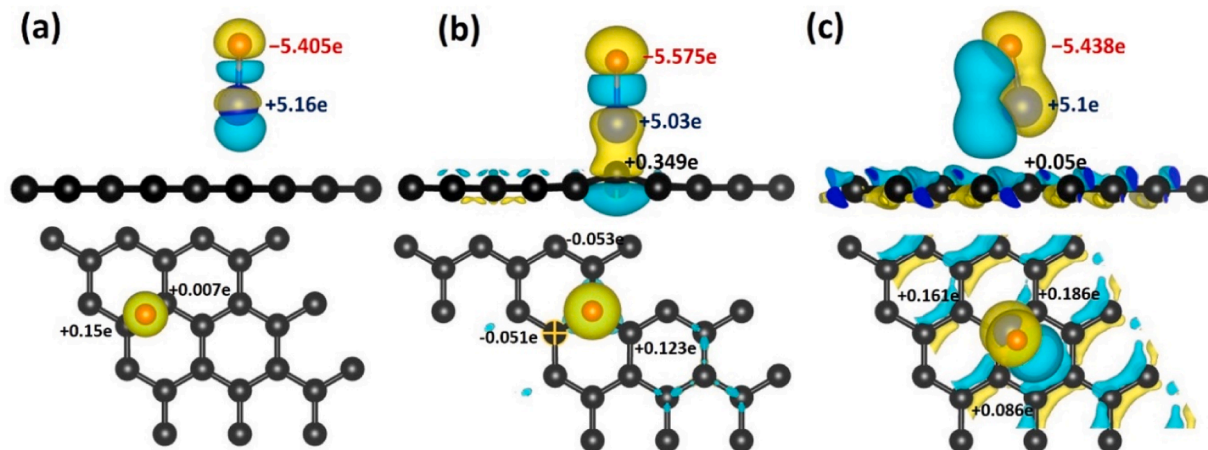
Fig. 6. (a) ZnO/G (Bridge site), (b) ZnO/G (Top site), and (c) ZnO/G (Hollow site) model adsorption structures; The isosurface value for the spin charge is 0.005 \text{ e/Å}^3 .
