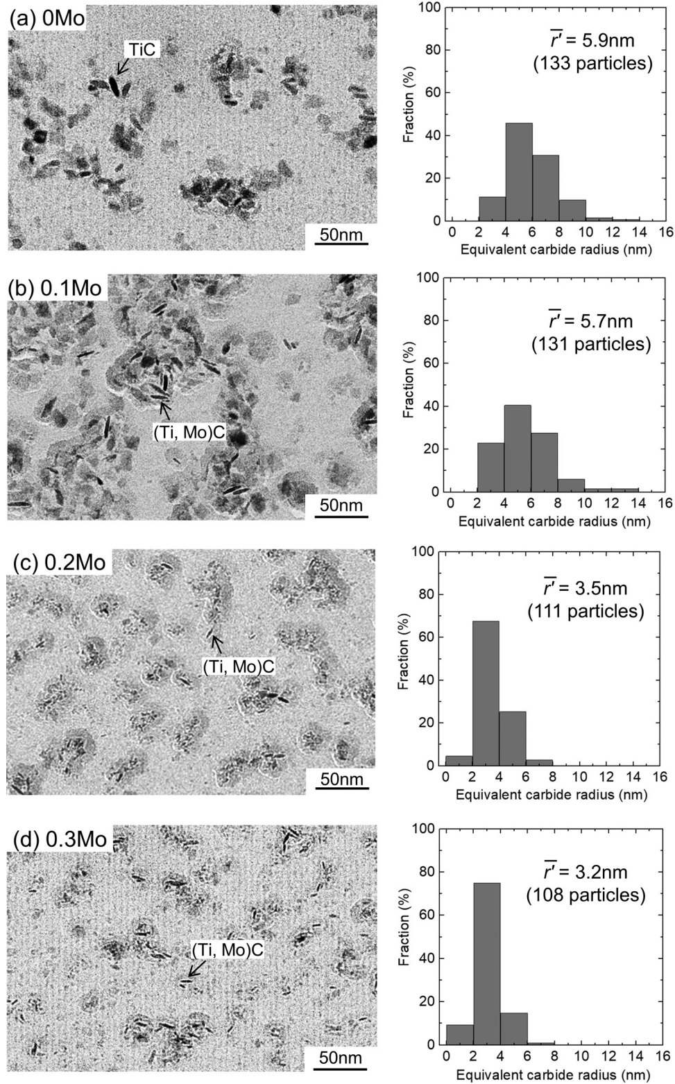
Fig. 8. Carbide distribution in carbon replicas and the corresponding statistical carbide radius for (a) 0Mo, (b) 0.1Mo, (c) 0.2Mo and (d) 0.3Mo alloys transformed at 660 °C for 16 h.
