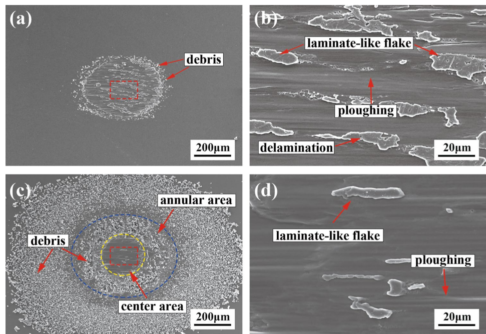
Fig. 10 SEM of worn scars of Ti6Al4V titanium alloy in GSR under a and b 4 \times 10^{-3} Pa, c and d 4 \times 10^{-1} Pa
