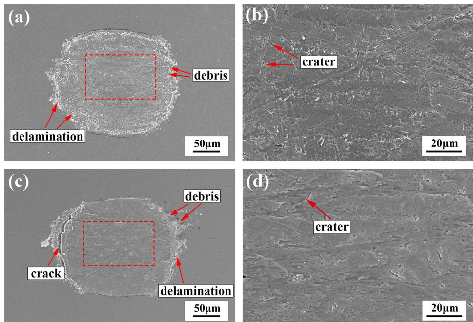
Fig. 8 SEM of worn scars of Ti6Al4V titanium alloy in MFR under a and b 4 \times 10^{-3} Pa, c and d 4 \times 10^{-1} Pa
