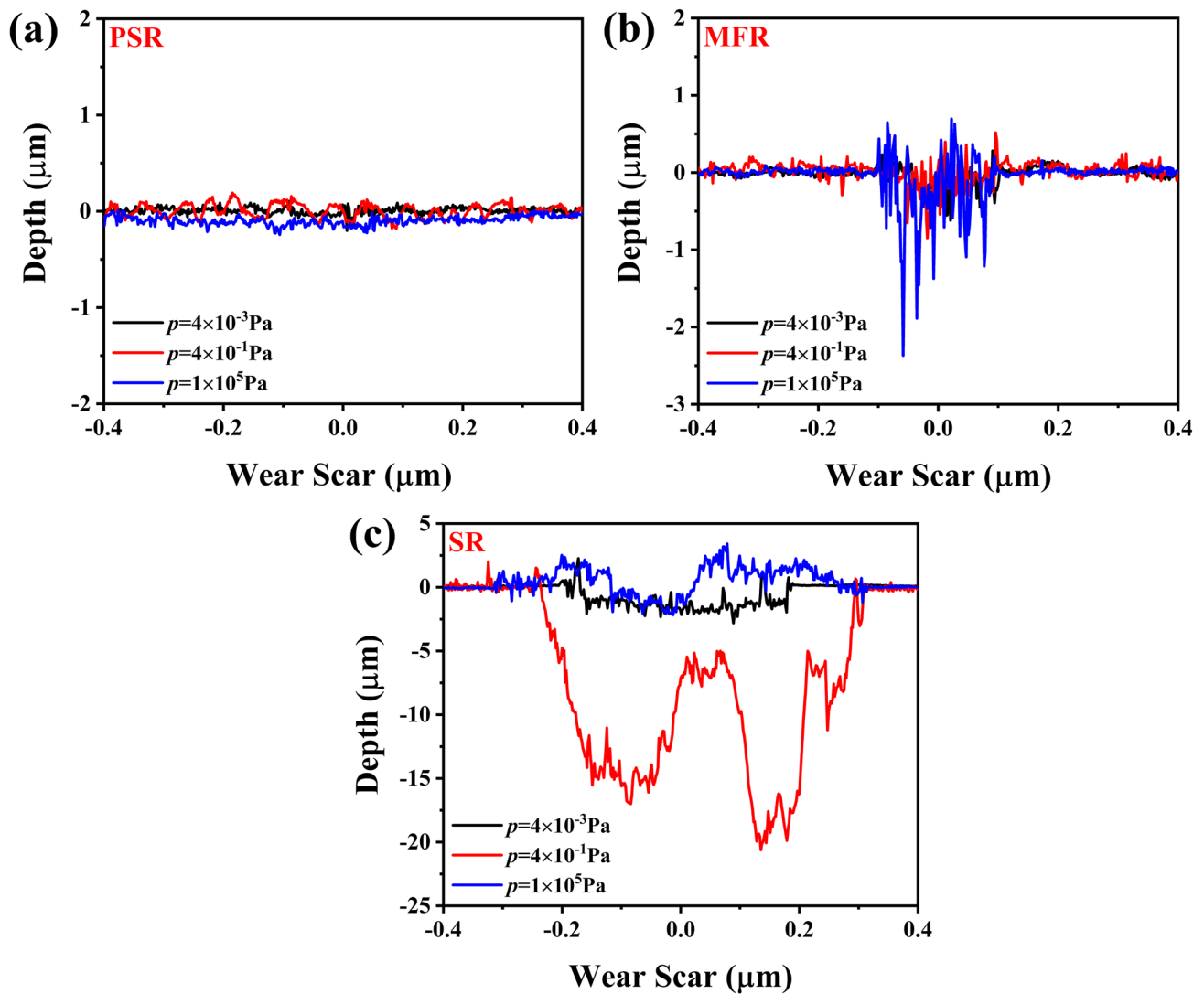
Fig. 15 Two-dimensional profiles of the worn scars of Ti6Al4V titanium alloy under different atmospheres in the different fretting regimes: a PSR, b MFR, and c GSR
