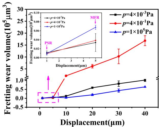
Fig. 14 The fretting wear volume evolutions of Ti6Al4V titanium alloy with the displacement amplitude in the different fretting regimes under different atmospheres (Note: the data points on wear volume in the 1 \times 10^5 Pa was reported in Ref. [27], and three data points on wear volume in the 4 \times 10^{-3} Pa was reported in Ref. [45].)
